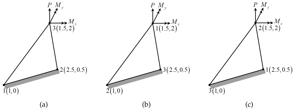
Fig. 4. Geometry, boundary, load and nodal numbering sequences for the isotropic element test
