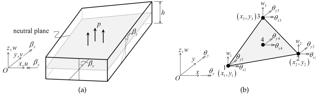
Fig. 1. (a) Mindlin-Reissner plate; (b) a 3-node triangular plate element with a bubble node
