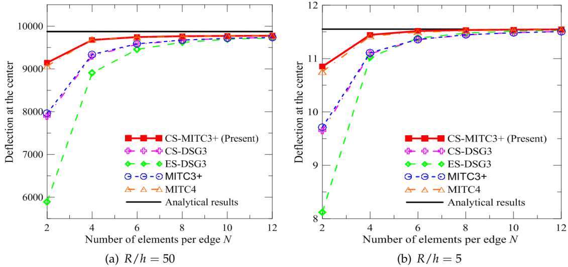
Fig. 10. Deflections at the center of the clamped circular plate
