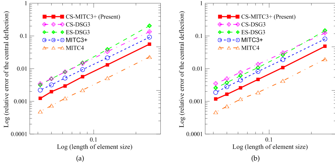
Fig. 6. Convergence rate of deflections at the plate center
