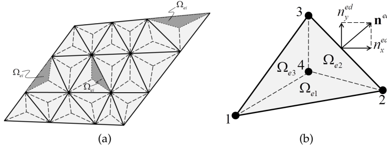
Fig. 2. (a) Mesh of the Mindlin-Reissner plate; (b) Definition of the subtriangular domains of a CS-MITC3+
