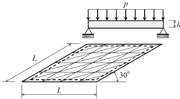
Fig. 7. Geometries, boundary conditions and 4 \times 4 meshes of the Morley's skew plate
