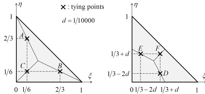
Fig. 3. Coordinates of typing points in the natural coordinates [14]
