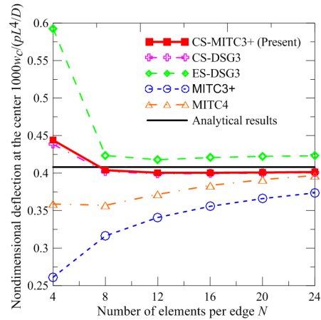
Fig. 8. Nondimensional deflections 1000w_c/(pL^4/D) at the center of the Morley's plate
