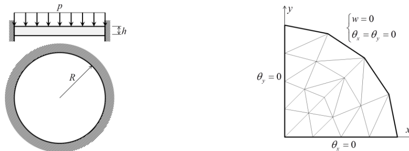
(a) Geometry, boundary and load of the circular plate (b) Symmetric model and N_x \times N_y = 4 \times 4 mesh
