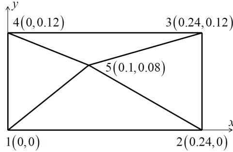
Fig. 5. Nodal coordinates of a mesh for the patch test
