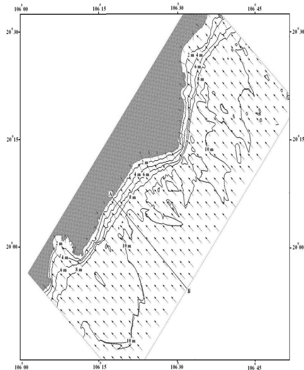
Fig. 4. The wave with returning period one hundred years at Hai Phong – Ninh Binh near shore zone
