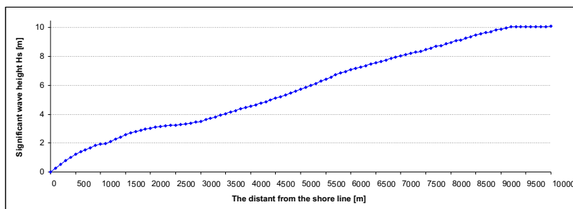
Fig. 5. Cross shore distribution of one hundred years wave heights form the point A to the point B (see the Fig. 4)
