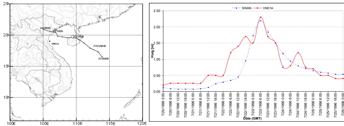
Fig. 1. Frankie’s path with the position of the buoy VN01A, a comparison of recoded and computed storm wave heights
