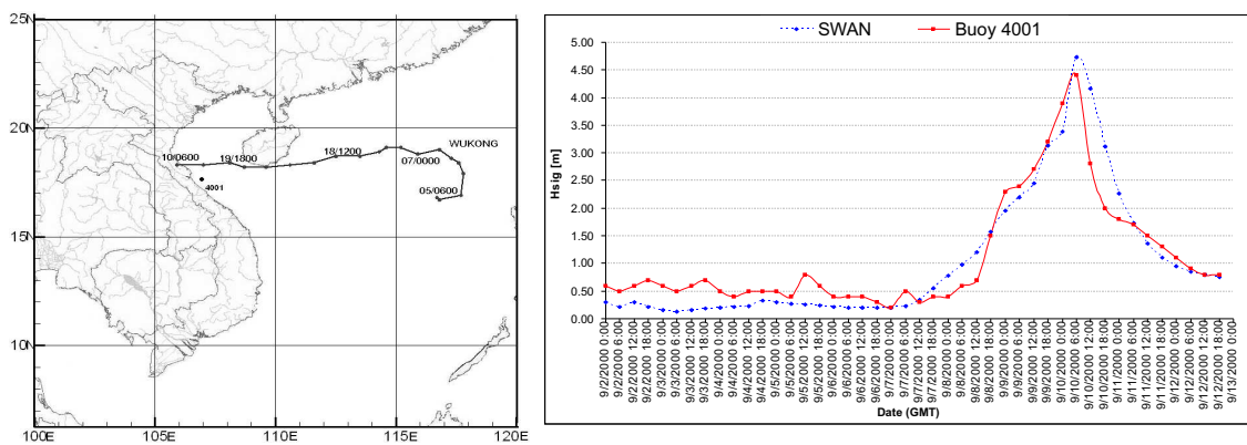
Fig. 2. Wukong’s path with the position of the buoy 4001, a comparison of recorded and computed storm waves
