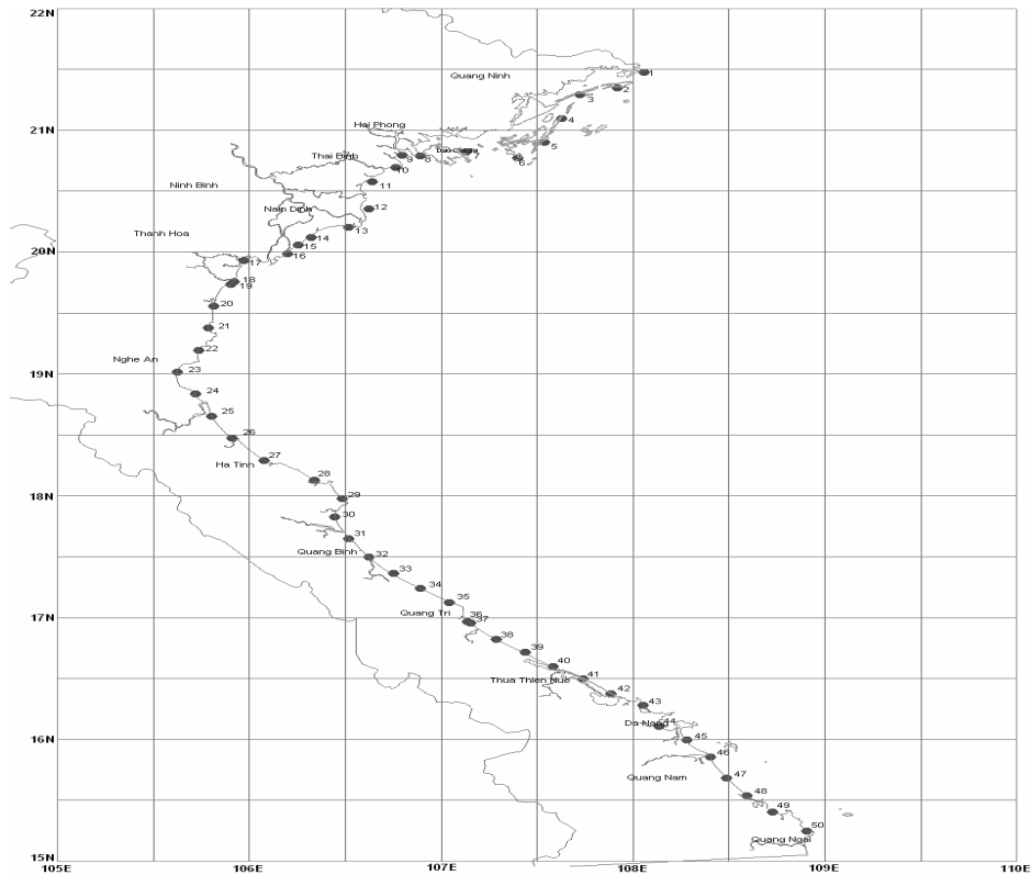
Fig. 3. The positions of the crossshore profiles for wave parameters computations
