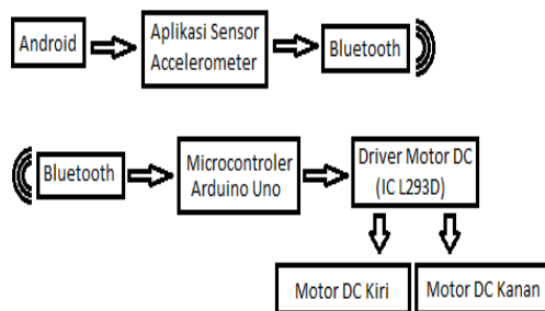
Gambar 2 Blok diagram
