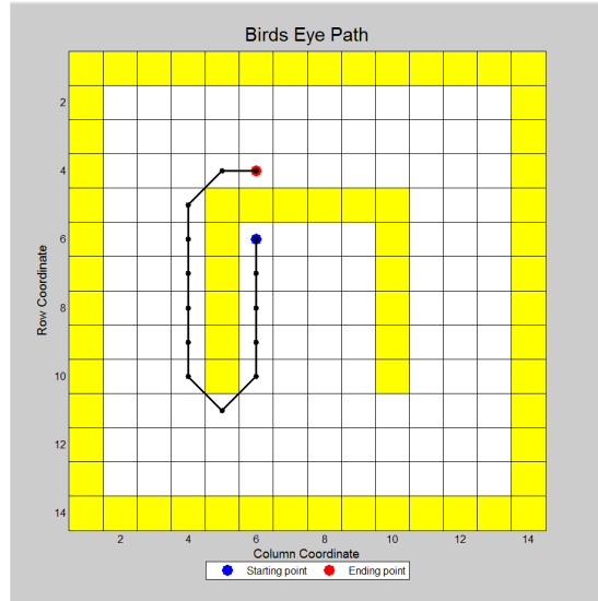
Figure 7.6. A* W/ Bird's Eye First Maze
