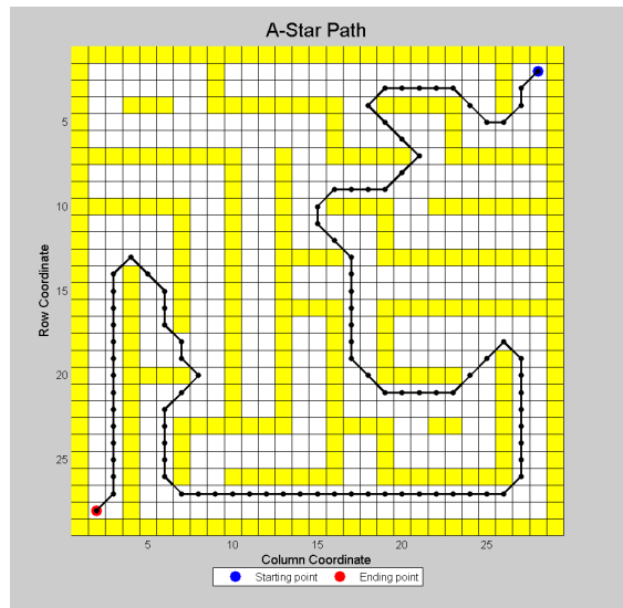
Figure 7.8. A* Second Maze
