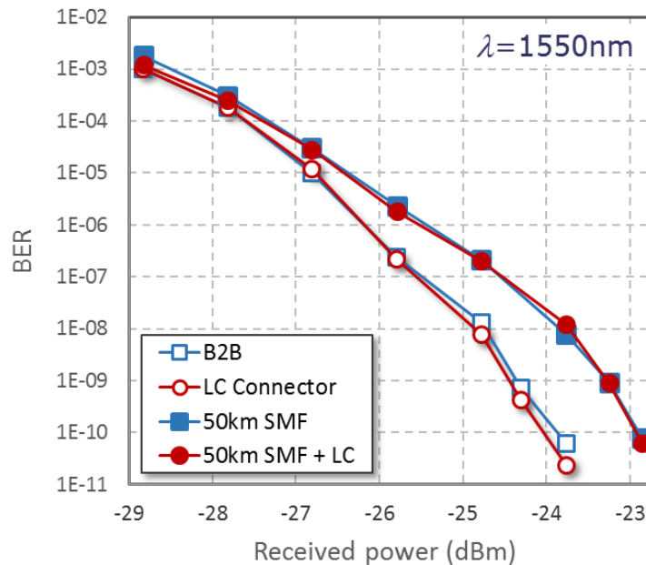
Fig. 4. Bit Error Rate of SMF GIF LC connections compared to both Back to Back and 50 km SMF 10 Git/s transmission.
