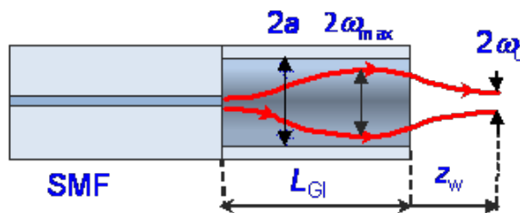
Fig. 1. Principle diagram of the SMF-GIF microlens.
