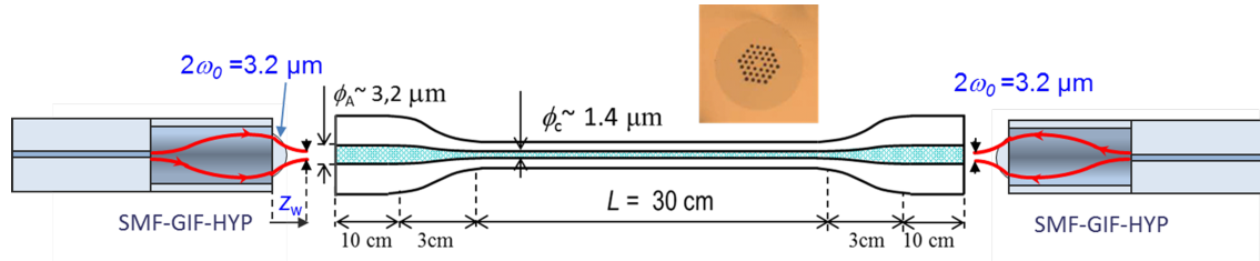
Fig. 5. Chalcogenide fiber and its micro-lensed fibers for coupling optimization.
