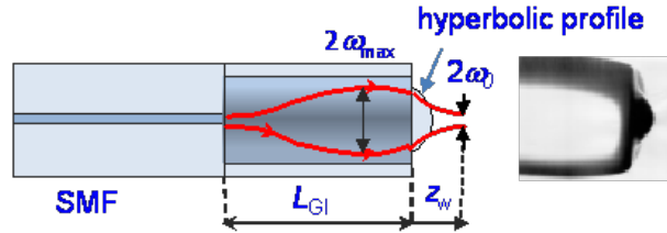
Fig. 2. Principle diagram of the SMF-GIF-HYP microlens.
