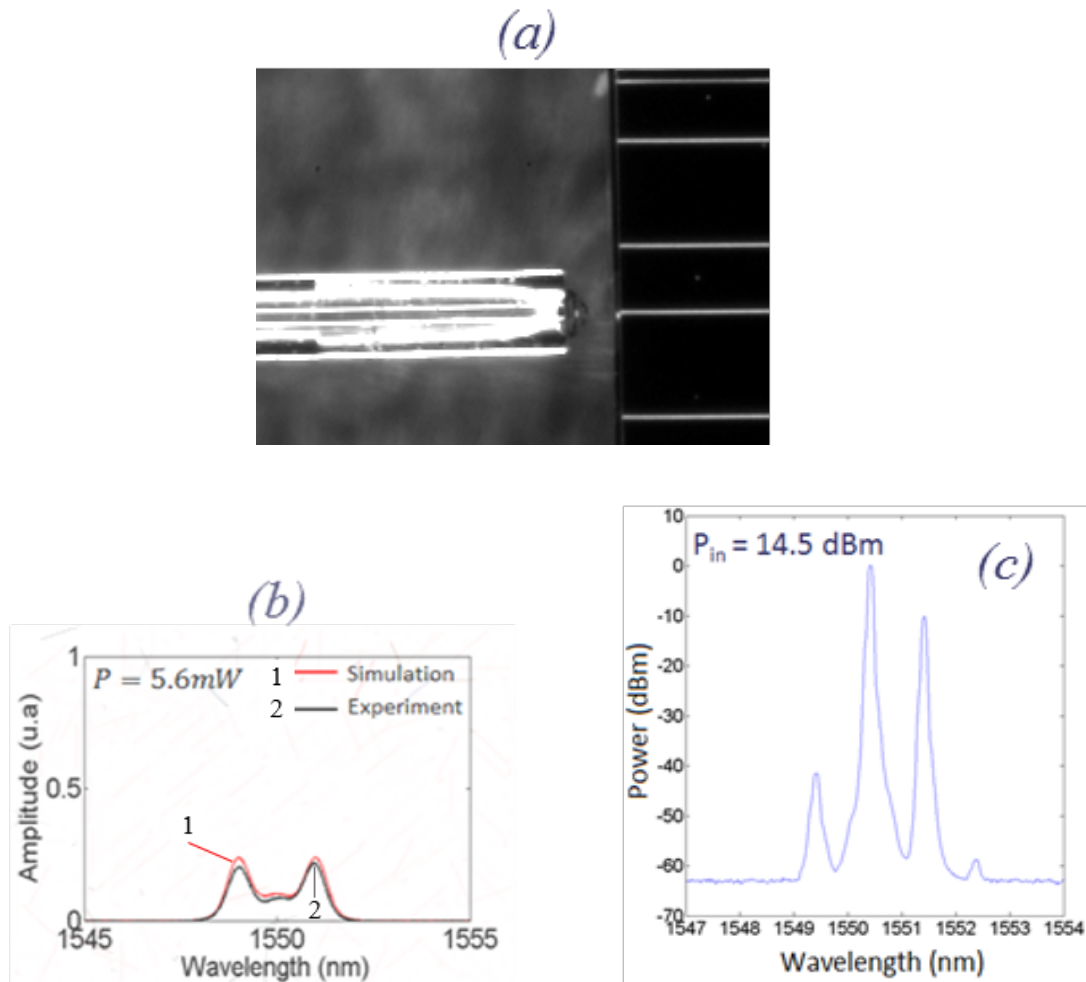
Fig. 7. (a) micro-lensed fiber and integrated waveguide photograph for coupling optimization; (b) Experimental spectrum measured at the waveguide output for 5.6 mW power to observe the SPM; (c) Experimental spectrum for a 1.1 cm long ChGs ridge waveguide to measure FWM.
