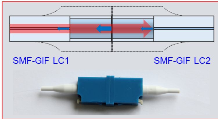
Fig. 3. SMF-GIF in LC connection.
