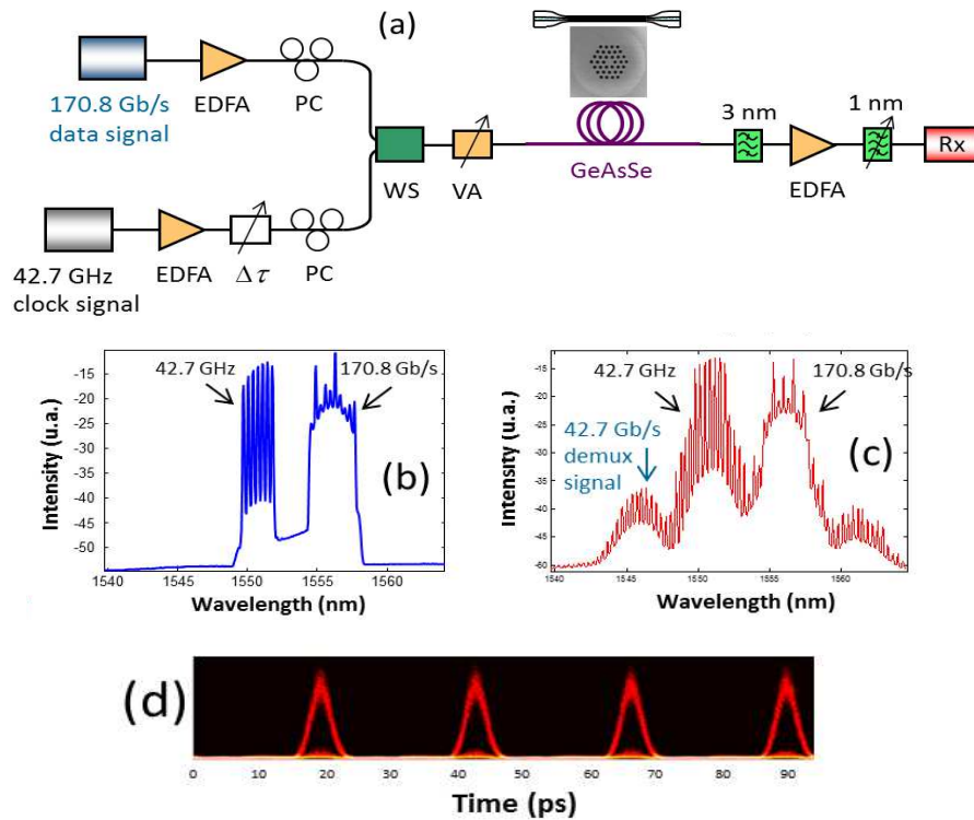
Fig. 6. Setup (a) and results on all-optical demultiplexing in a chalcogenide fiber (b), (c) and (d).
