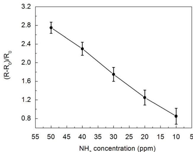
Fig. 5. Sensitivity of P3GC sensor vs. ammonia concentration.
