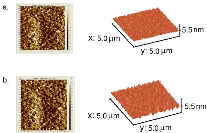
Fig. 1. AFMs of a pure P3HT (a) and P3GC (b) film annealed at 120°C for 2 hours.
