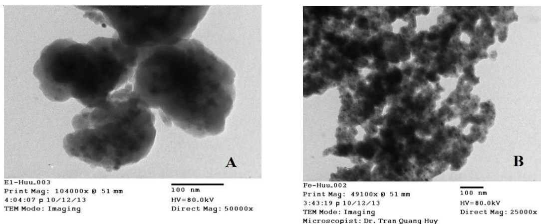
Fig. 3. TEM images in Fe 3 O 4 .SiO 2 -Alcalase (A) and Fe 3 O 4 .SiO 2 (B)
