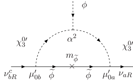
Fig. 1. Feynman diagram for the process \phi \rightarrow \nu_R \nu_R
