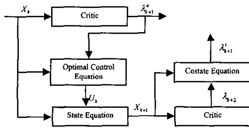
Figure 2: Single Network Adaptive Critic Scheme
