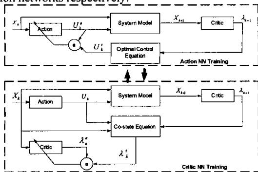
Figure 1: Adaptive Critic Network Training
