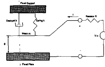
Figure 3: Electrostatic Actuator
