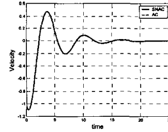
Figure 6: SNAC/AC State 3 trajectories
