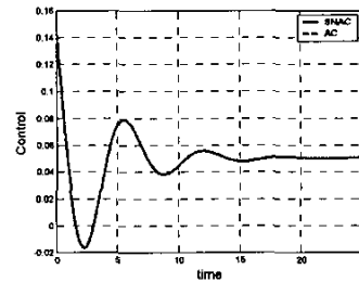
Figure 7: Associated control trajectories
