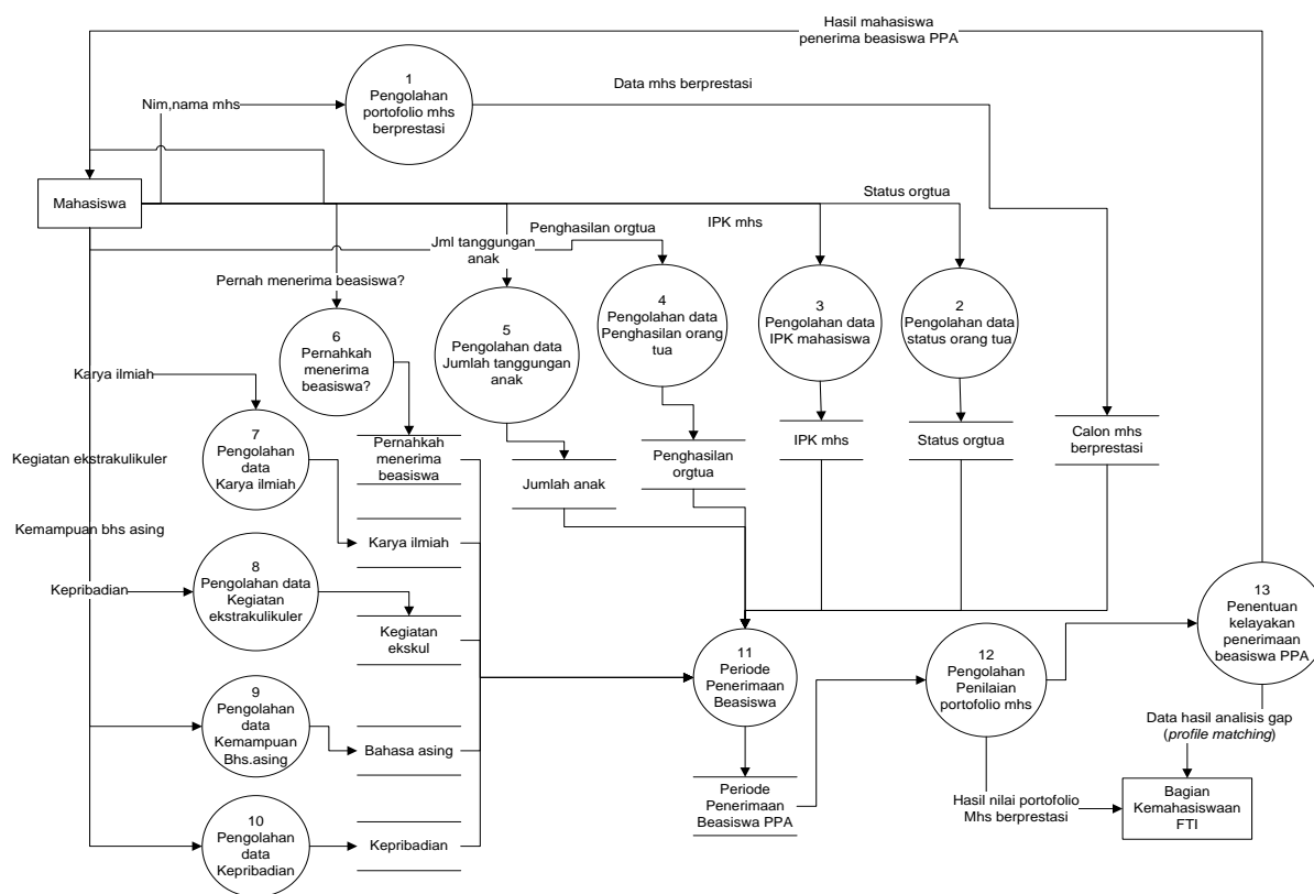
Gambar 2. DFD Level 0
