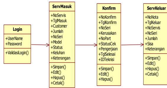
Gambar 2.2 Class Diagram
