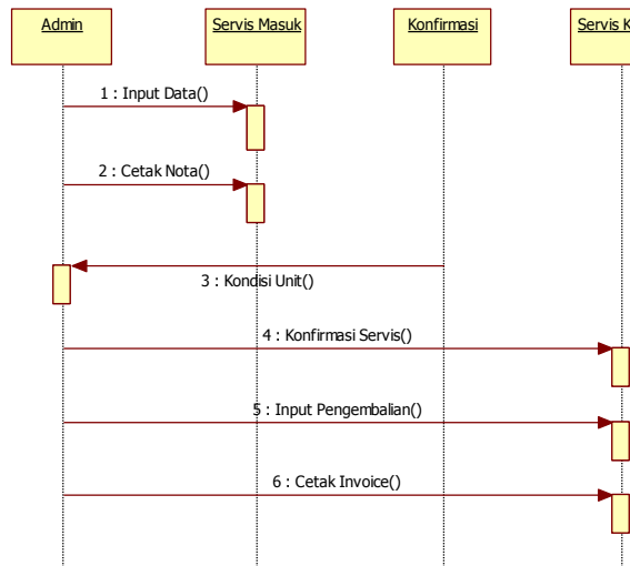
Gambar 2.5 Sequence Daiagram
