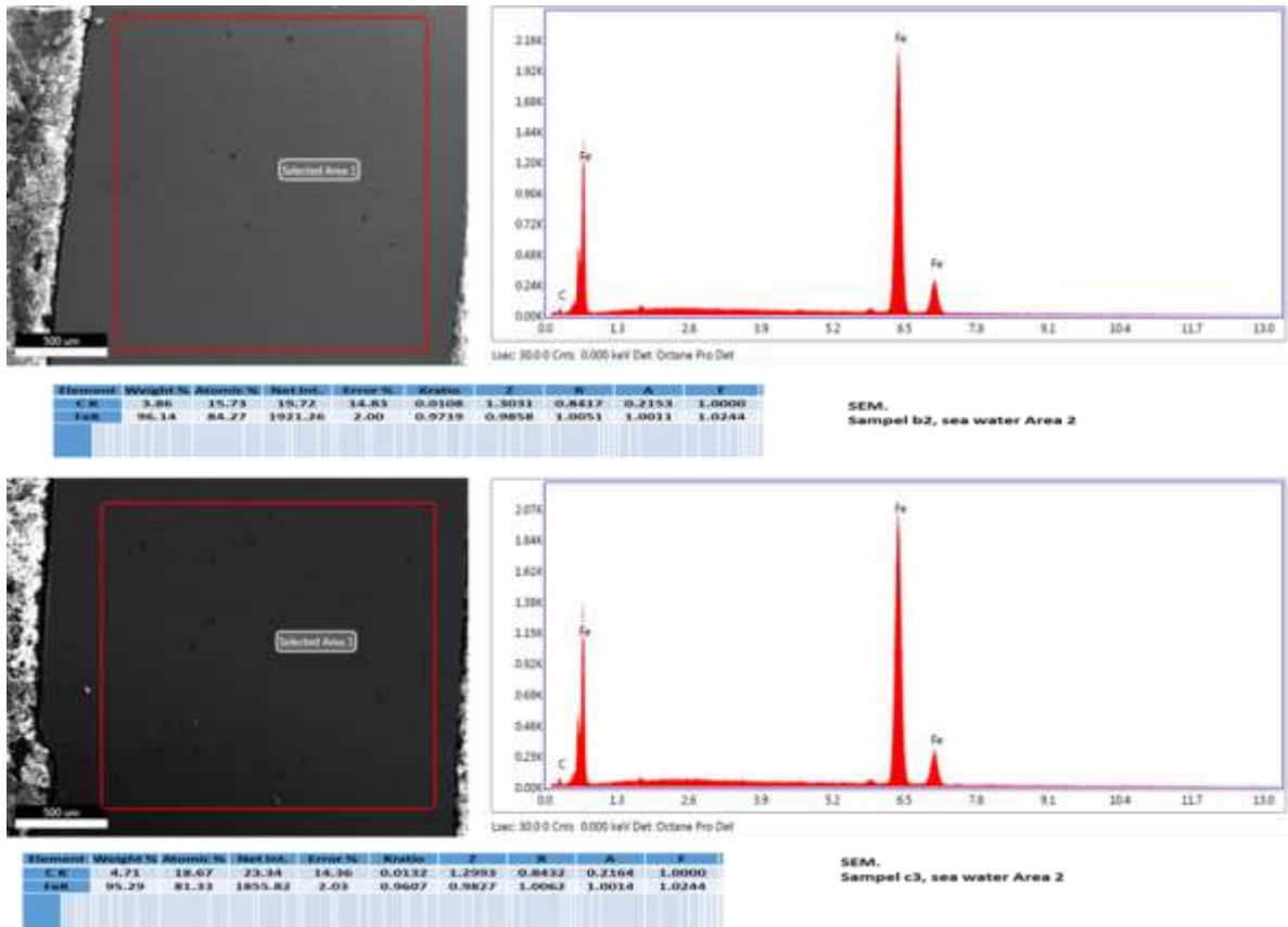
Figure 10. Result SEM-EDS for b2 and c3 samples.
