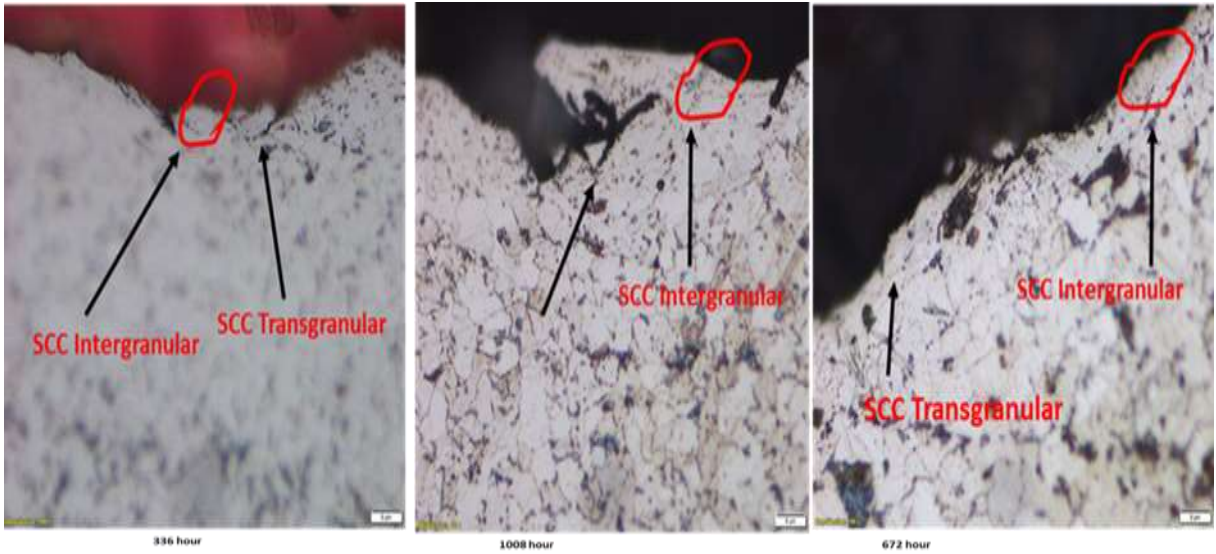
Figure 6. Results of microstructure.
