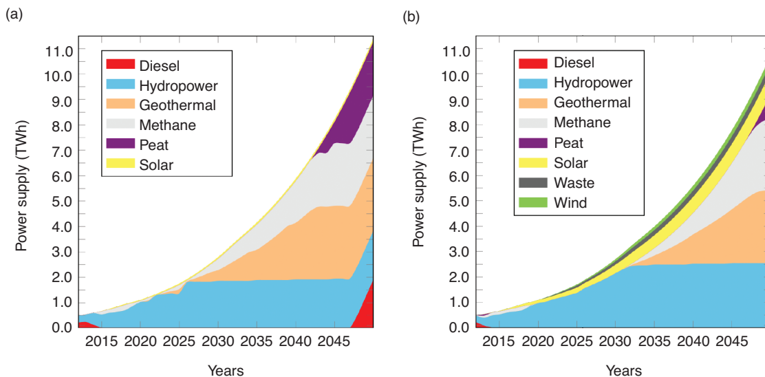
Figure 3: Electricity supply by resource under no climate change considerations
