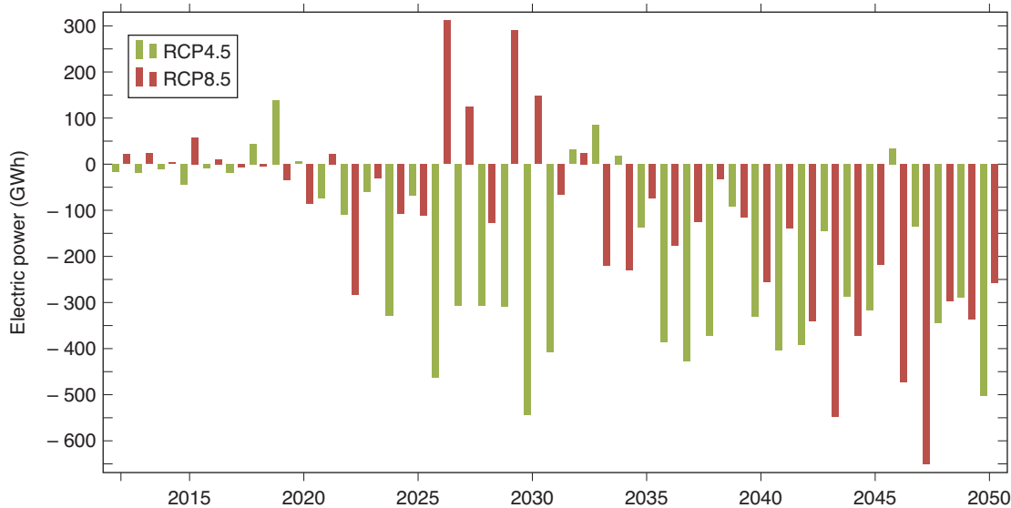
Figure 2: Hydropower generation anomalies between 2012 and 2050
