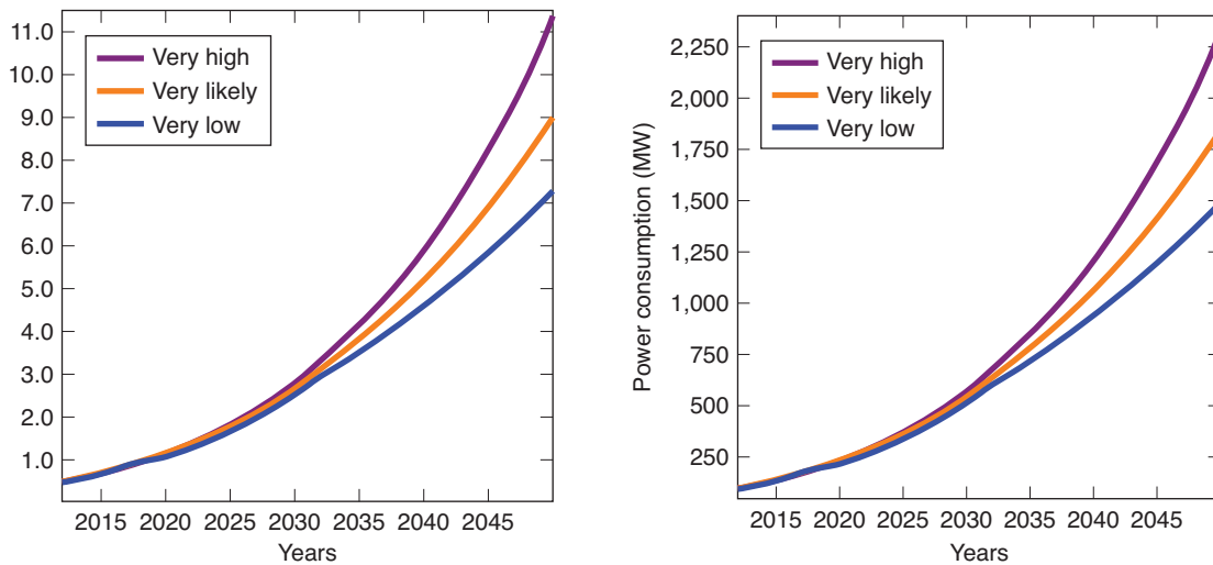
Figure 1: Electricity generation (left) and peak power (right) requirements
