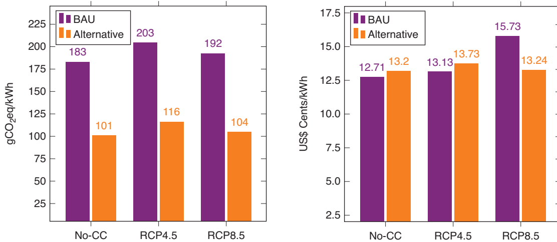
Figure 6: Average emissions and generation cost per kWh for the 2012–2050 period
