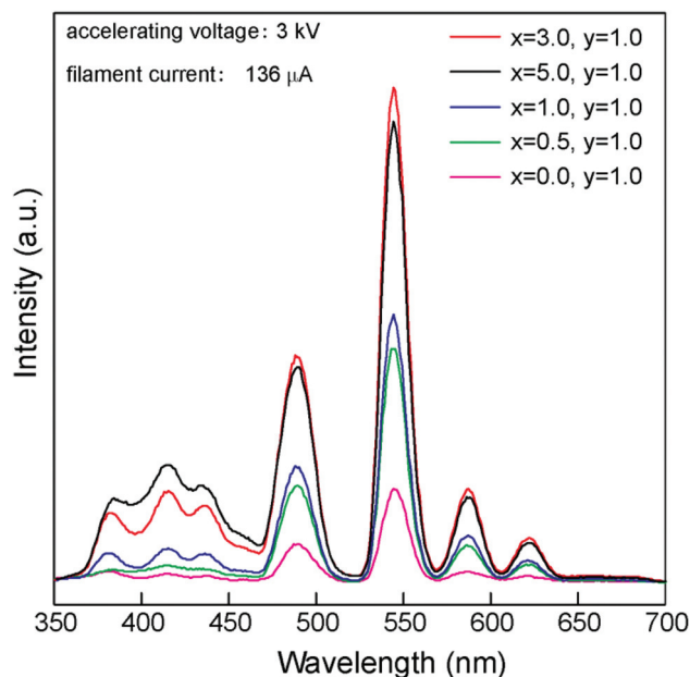
Fig. 6 CL spectra of \text{C12A7}:x\% \text{Ce}^{3+}, 1.0\% \text{Tb}^{3+} phosphors annealed at 1300^\circ\text{C} for 6 hours in a reducing atmosphere under low-voltage (3 kV) electron beam excitation.
