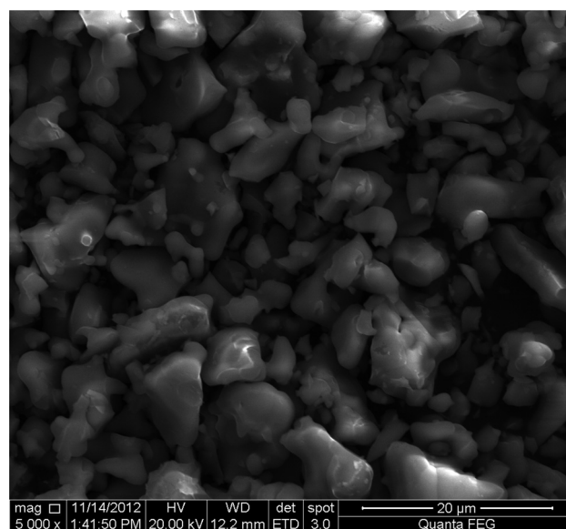
Fig. 9 SEM image of C12A7:3.0% Ce 3+ , 1.0% Tb 3+ annealed at 1300 °C for 6 hours under a reducing atmosphere.
