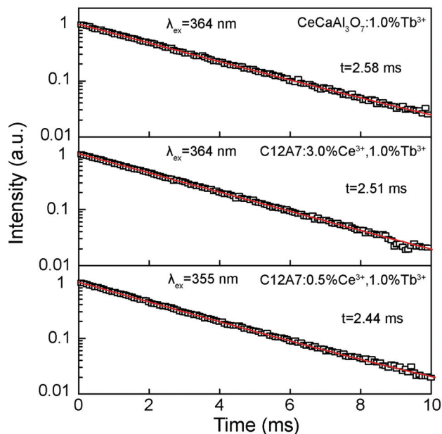
Fig. 12 Decay curves of Tb 3+ emission monitored at 543 nm for phosphors C12A7:0.5% Ce 3+ , 1.0% Tb 3+ , C12A7:3.0% Ce 3+ , 1.0% Tb 3+ , and CaCeAl 3 O 7 :1% Tb 3+ . The red line represents the data best fitted using a single exponential function.
