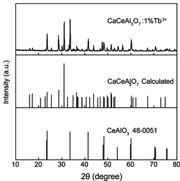
Fig. 4 XRD patterns of CaCeAl 3 O 7 :1% Tb 3+ containing CeAlO 3 and the calculated CaCeAl 3 O 7 .
