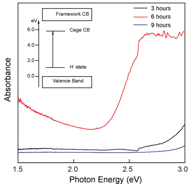
Fig. 8 The absorption spectra of C12A7:3.0% Ce 3+ , 1.0% Tb 3+ annealed at 1300 °C for different times (3, 6, and 9 hours).
