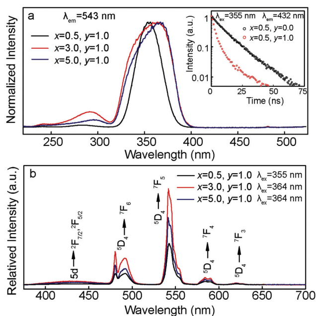
Fig. 3 Excitation (a, normalized) and emission spectra (b) of the C12A7: x % Ce 3+ , 1.0% Tb 3+ annealed at 1300 °C for 6 hours under a reducing atmosphere. The inset shows decay curves of Ce 3+ under 355 nm excitation.
