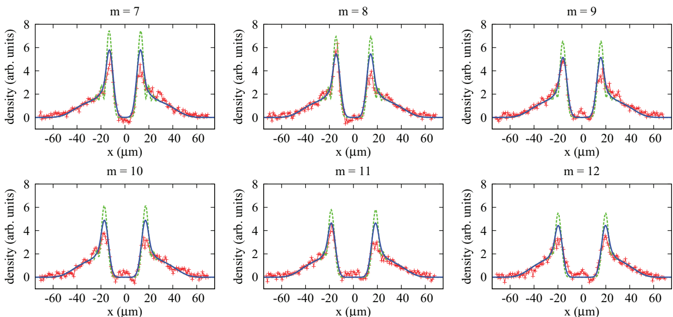
FIG. 6. (Color online) Comparison of the cut through of the condensate optical density data after direct release and 10 ms TOF with GP simulations for initial circulations m = 7, \dots, 12 .
