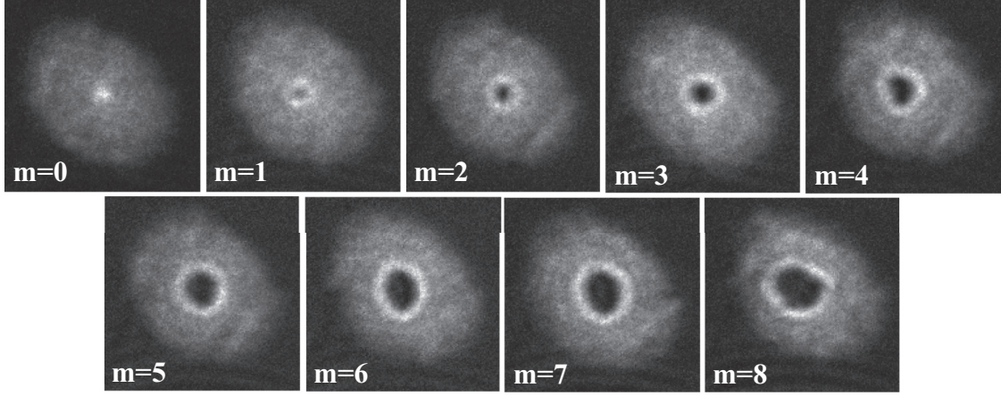
FIG. 4. Time-of-flight images of the condensate after ramp down and release from the trap and 10 ms TOF. Each image is labeled with the circulation m that was determined by analysis of hole size as shown in Fig. 2.
