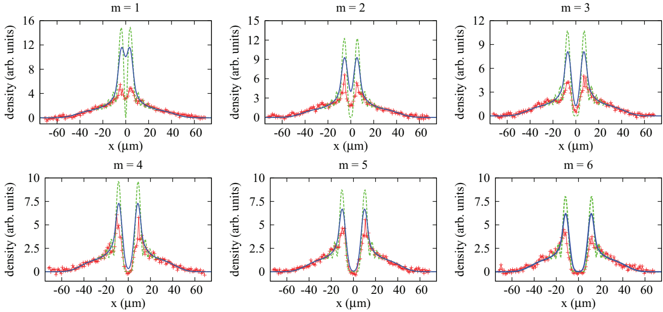
FIG. 5. (Color online) Comparison of the cut through of the condensate optical density data (shown as individual points connected with a solid red line) after direct release and 10 ms TOF with GP simulations for initial circulations m = 1, \dots, 6 . Two theoretical curves appear in each graph. The dotted (green) curve is the result of evolving the 3D TDGPE. The solid (blue) curve is a cut through of the TDGPE prediction convolved with a Gaussian having a 4 \mu\text{m} 1/e^2 radius to account for the finite resolution of the experimental instrument.
