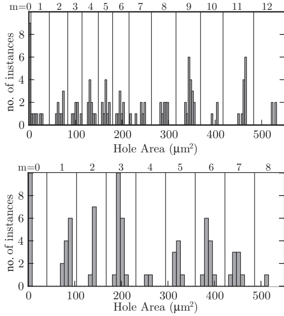
FIG. 2. Circulation of stirred condensates was determined experimentally from the distribution of hole sizes in the expanded cloud. These distributions are shown in the histograms above for the direct-release case (upper) and for the ramp-and-release cases (lower). The winding number m assigned for a given hole area is labeled for each bin.
