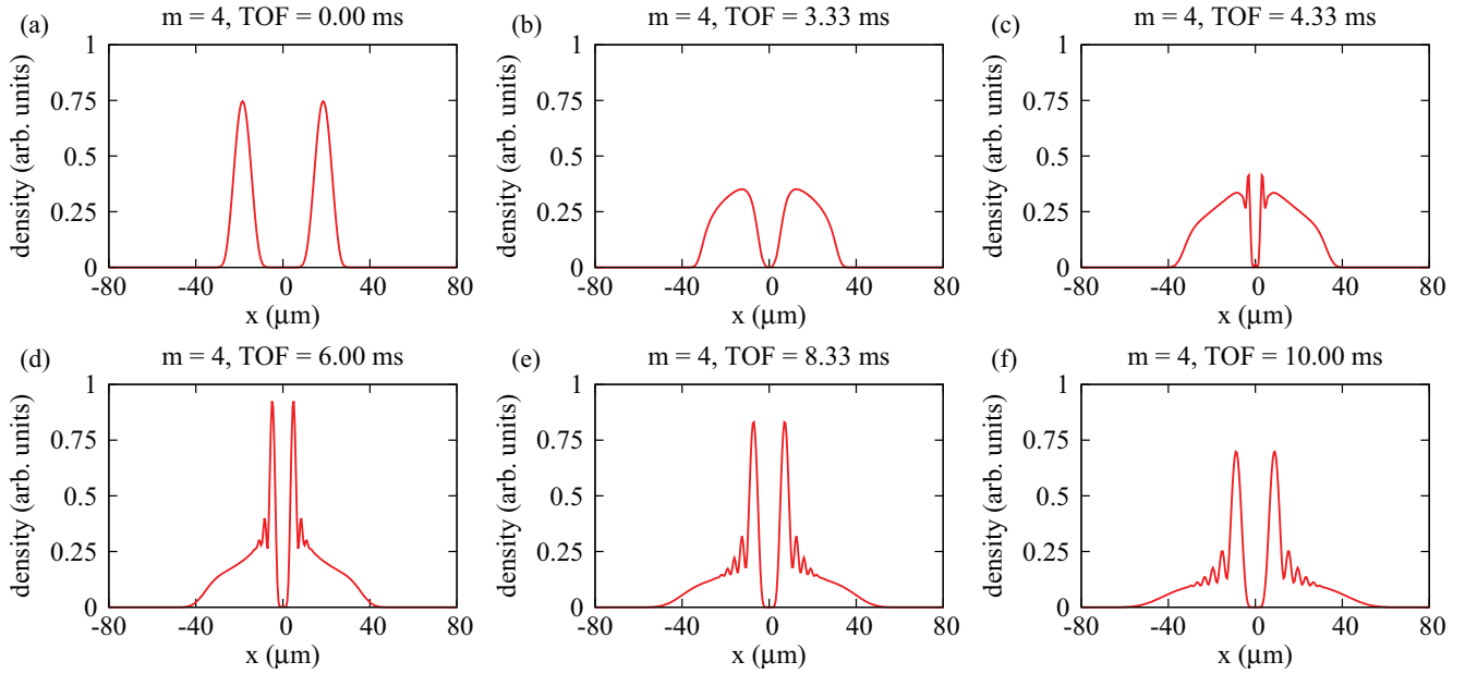
FIG. 8. (Color online) Sequence of cut throughs of the optical density as a function of time after direct release depicting the dynamics of the expansion. The initial condensate was phase imprinted with four units of angular momentum.
