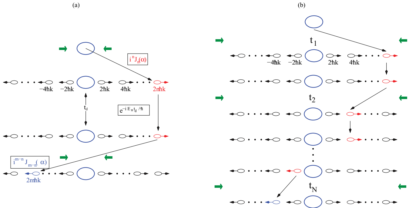
FIG. 1. (Color online) (a) The final distribution of the condensate atoms over the momentum states after the application of two standing-wave pulses separated by an interval can be understood in terms of interfering quantum pathways. The amplitude for the system to jump from the initial zero-momentum state at the top to the final state at the bottom along the path shown is the product of the amplitudes (shown in boxes) for the three legs that compose the path. The total amplitude is a coherent summation of this composite single-path amplitude over all possible paths. (b) The general case of N pulses is illustrated. We assume that pulse 1 is applied at t_1 , pulse 2 at t_2 , etc.
