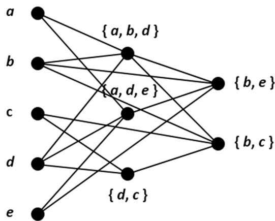
Figure 6. A 3-partite set intersection graph. Singleton vertices that represent a, b, c, d, and e comprise one partite set. Subset vertices that represent \{a, b, d\}, \{a, d, e\}, and \{d, c\} comprise a second partite set. A third partite set consists of subset vertices that represent \{b, e\} and \{b, c\} .
