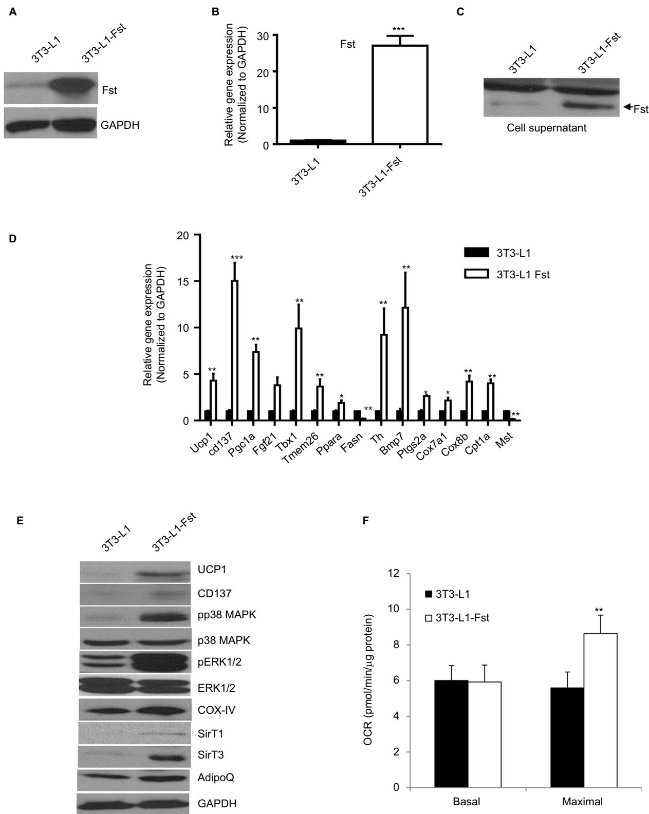
Figure 2 Comparative analysis of Fst expression, key brown/beige related markers and oxygen consumption in Fst overexpressing 3T3-L1 Fst and 3T3-L1 cells. Analysis of relative Fst protein (A), gene expression (B), and Fst release in cultured medium (30 \mu l supernatant) (C) in 3T3-L1 and 3T3-L1 Fst grown under normal growth conditions. (D) Quantitative gene expression analysis of key markers involved in adipose browning, mitochondrial biogenesis pathway in cells allowed to differentiate under standard adipogenic differentiation conditions for 9 days. (E) Western blot analysis of key proteins involved in adipose browning and regulation of key signaling pathway involved during the process in differentiated 3T3-L1 and 3T3-L1 Fst cells. (F) Analysis of OCR in differentiated 3T3-L1 and 3T3-L1 Fst cells after 9 days using Seahorse Bioscience XF24 extracellular flux analyzer. Data are expressed as mean \pm SD. * P \leq 0.05 , ** P \leq 0.01 , and *** P \leq 0.001 . (n=3).
