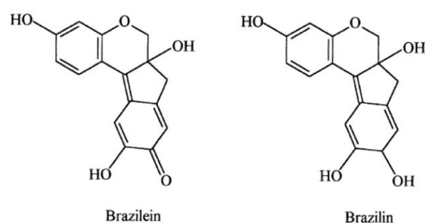
Gambar 1.1. Struktur kimia brazilin (a) dan brazilein (b) (Wongsookin 2008)
