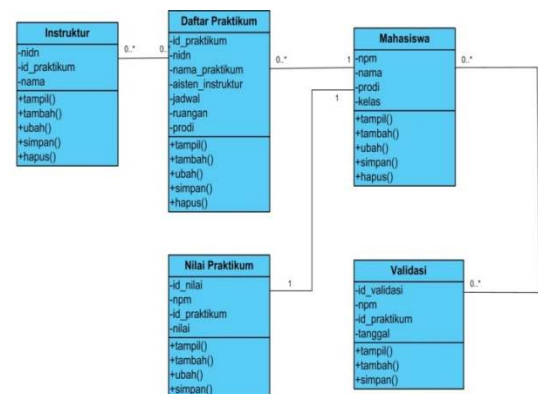
Gambar 6. Class Diagram
