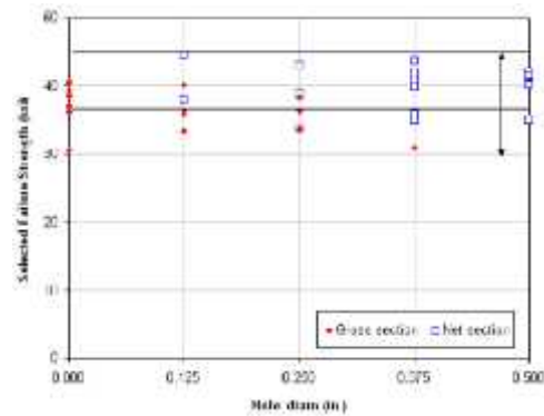
Fig. 6 Variation of notch strength with hole diameter (Feraboli et.al, 2009)
