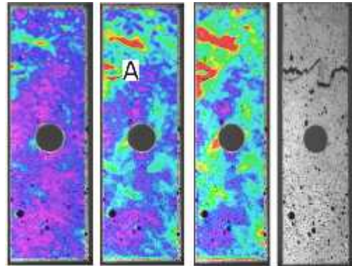
Fig.9 Example of DIC full-field strain plot (Bond et.al, 2010)
