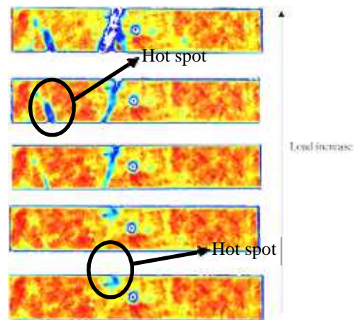
Fig. 7 Ultrasonic imaging up to failure for DCFC specimen with hole (Feraboli et.al, 2009)
