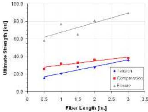
Fig. 3 Ultimate strength of DCFC for different load type (Feraboli et.al, 2009)
