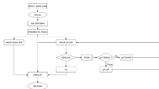
Gambar 16 Flow chart program
