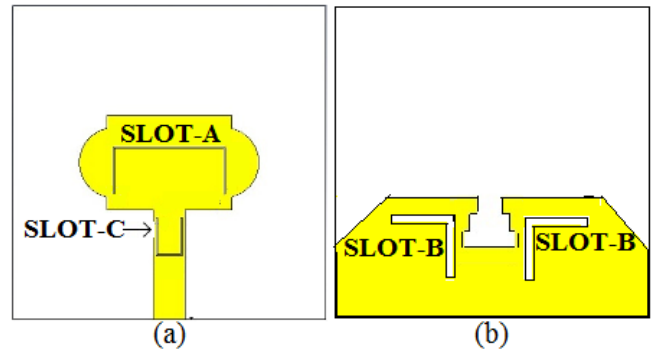
Figure 5: Proposed triple band notch hammer-shaped Antenna-D geometry (a) top side, and (b) bottom side.
