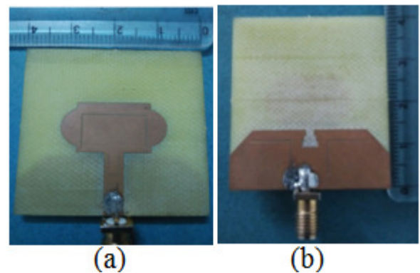
Figure 6: Proposed fabricated triple band notch hammer-shaped Antenna-D (a) top side, and (b) bottom side.
