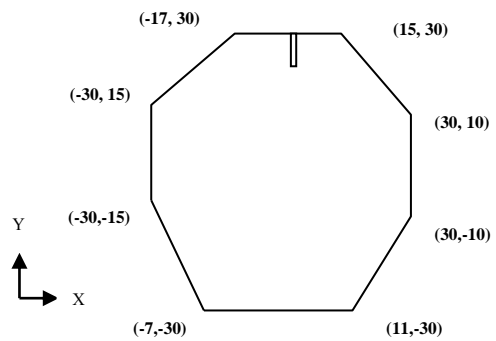
Fig. 1.11 Polygon shaped patch Antenna 3-Topology
