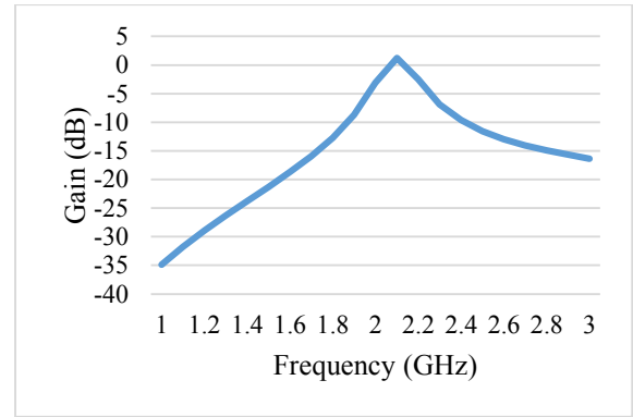
Fig.1.15 Gain vs Frequency relationship of the Antenna 3
