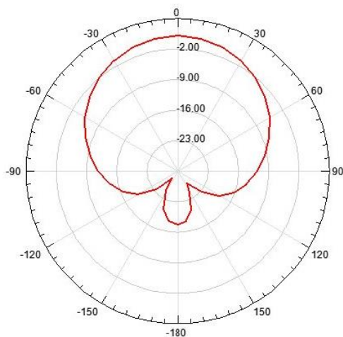
Fig. 1.14 2D Radiation Pattern of the Antenna 3
