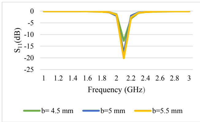
Fig 1.13 S 11 Response of the Antenna 3
