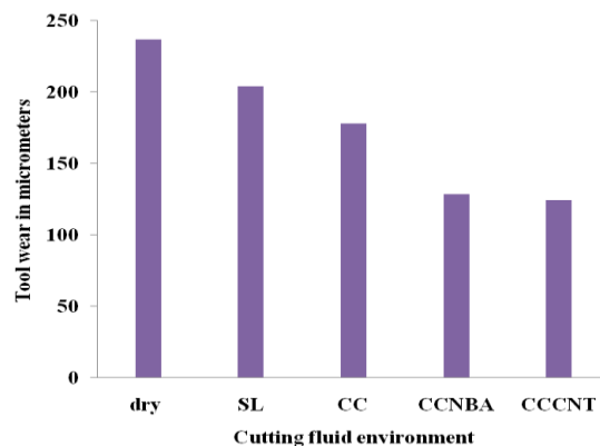
Fig. 4 Variation of Tool wear with cutting fluid environment (Speed : 560 rpm; Feed : 0.14mm/rev; Depth of cut : 0.5mm; NPI : 0.25%)
