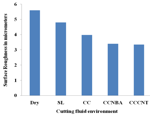
Fig. 5 Comparison of Surface Roughness in different lubricant environments (Speed : 560 rpm; Feed : 0.14mm/rev; Depth of cut : 0.5mm; NPI : 0.25%)
