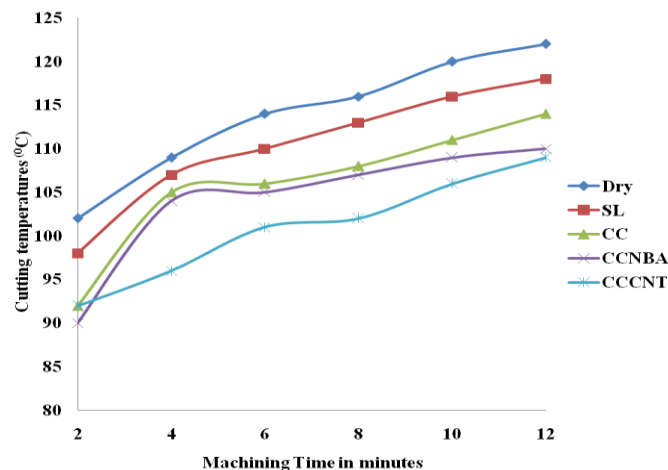
Fig.2 Variation of Cutting temperatures with machining time (Speed: 560 RPM; Feed: 0.14mm/rev; Depth of Cut : 0.5mm; NPI : 0.25%)
