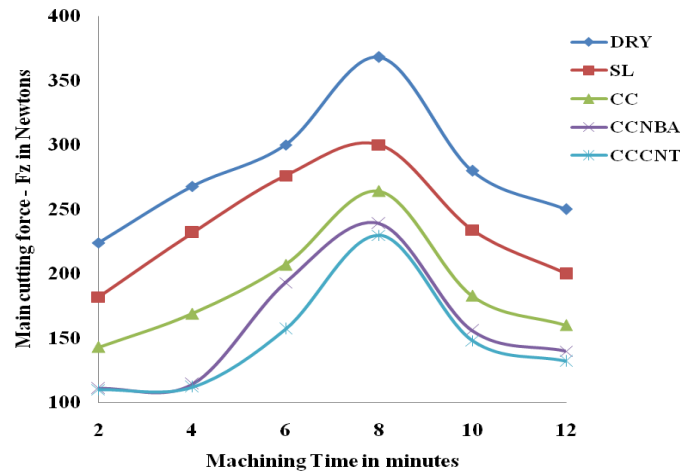
Fig. 3 Variation of Cutting Force with machining time (Speed : 560 rpm; Feed : 0.14mm/rev; Depth of cut : 0.5mm; NPI : 0.25%)
