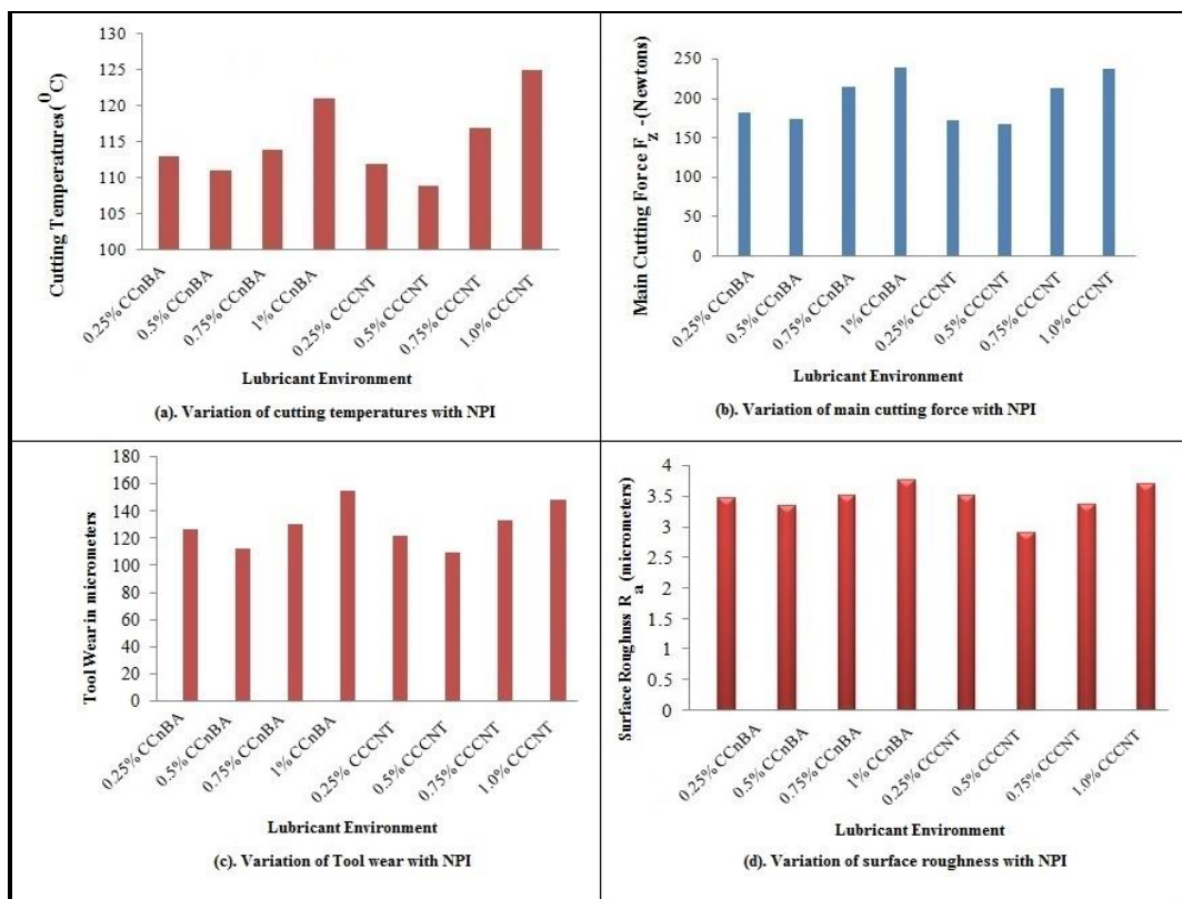
Fig. 6 Variation in machining performance with NPI (Speed : 560 rpm; Feed : 0.14mm/rev; Depth of cut : 0.5mm)
