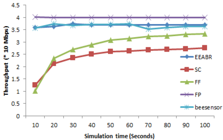
Fig. 2 Throughput vs. simulation time
