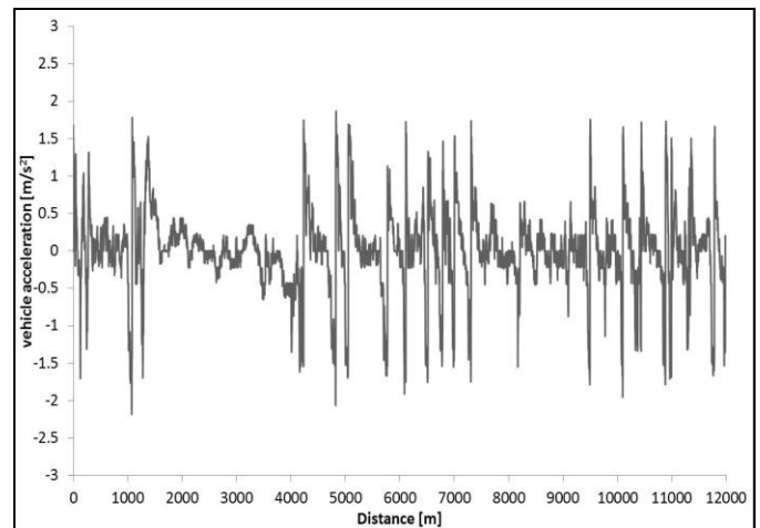
(c) computed acceleration vs. space
