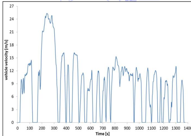
(a) prescribed velocity vs. time
