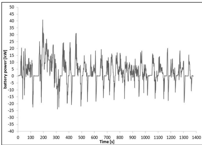
(c) measured battery power vs. time
