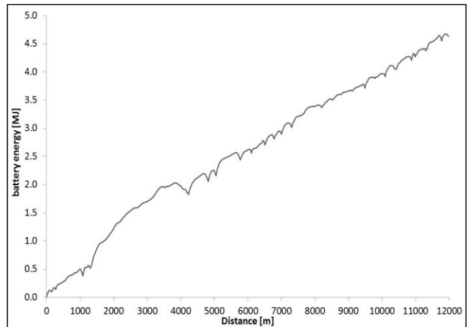
(b) measured net battery energy
