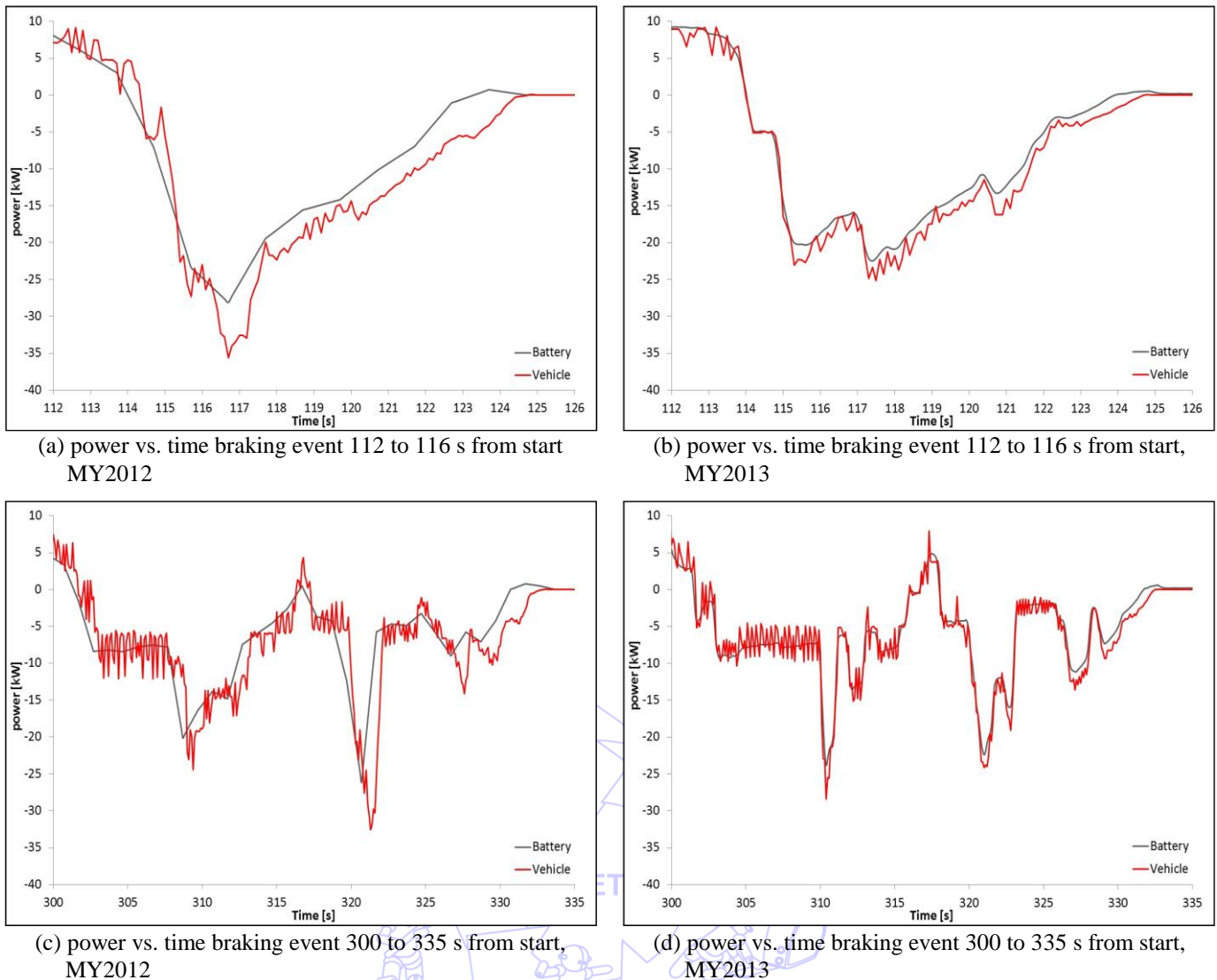
Fig. 5 UDDS, Test cell temperature 72 F, Hot Start, Computed vehicle reference propulsive (positive) and braking (negative) power P_w(t) , and measured HV battery power out (positive) and in (negative) P_{HV}(t)
