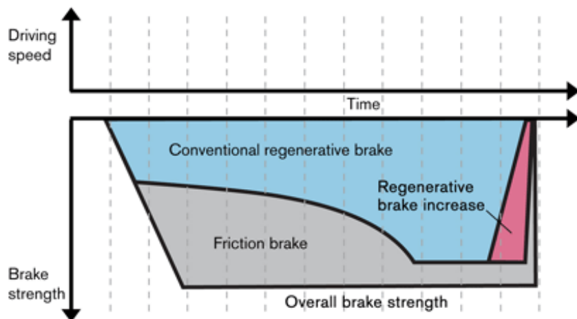
(b) Regenerative and friction brakes intensity, brake strength – time map (image from [7]), MY2013 vs. MY2012
