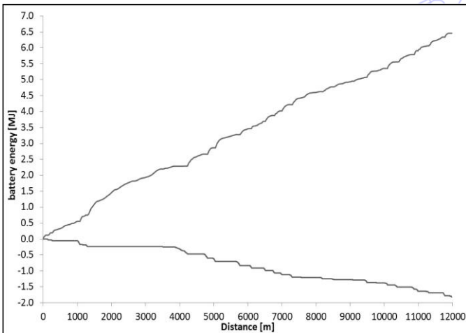
(a) measured energy from and to battery
