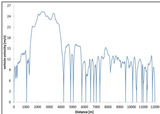
(b) prescribed velocity vs. space
