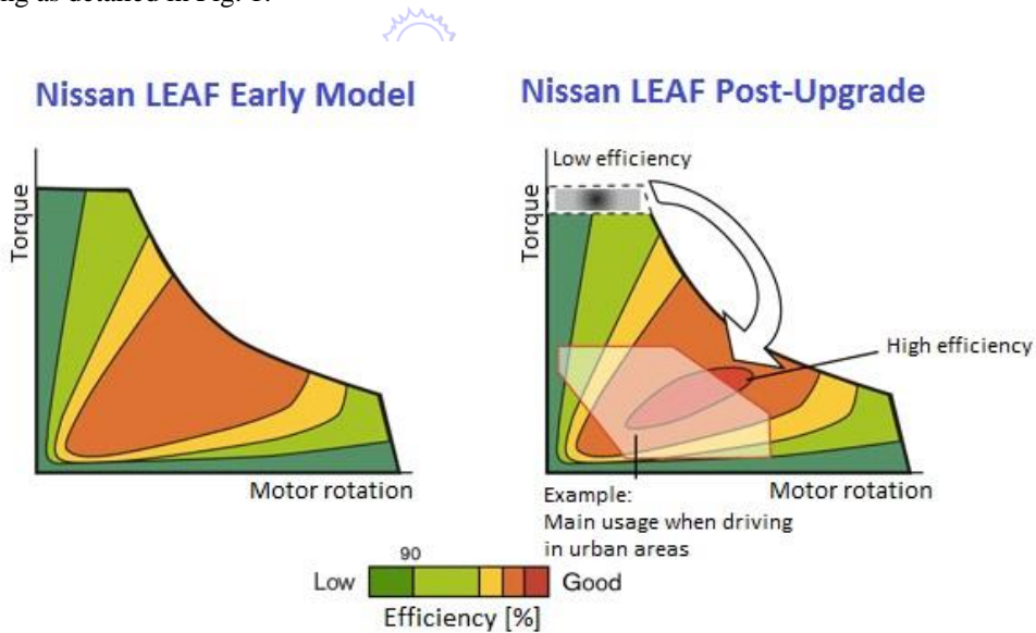
(a) Operating points of the motor, torque – speed map (image from [7]), left MY2012, right MY2013
