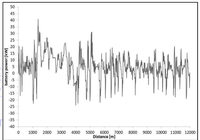
(d) measured battery power vs. space
