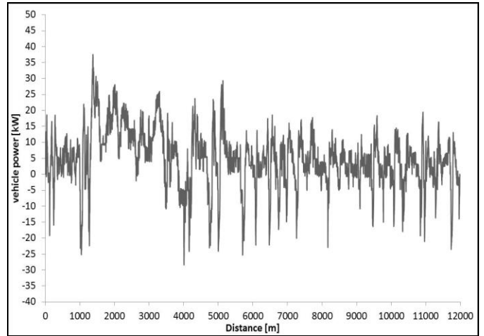
(b) computed vehicle reference propulsive and braking power vs. space
