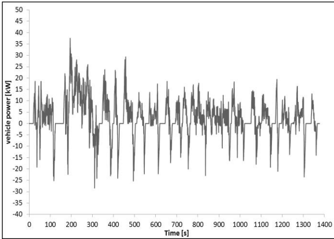
(a) computed vehicle reference propulsive and braking power vs. time
