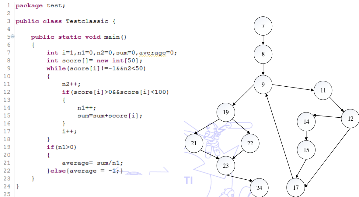
Fig. 10 Java source code of average score
