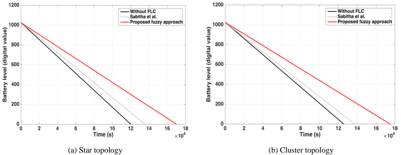
Fig. 7 Battery consumption comparison
