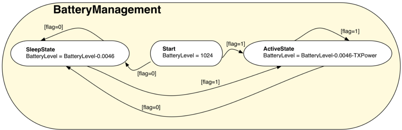
Fig. 6 Battery consumption flowchart
