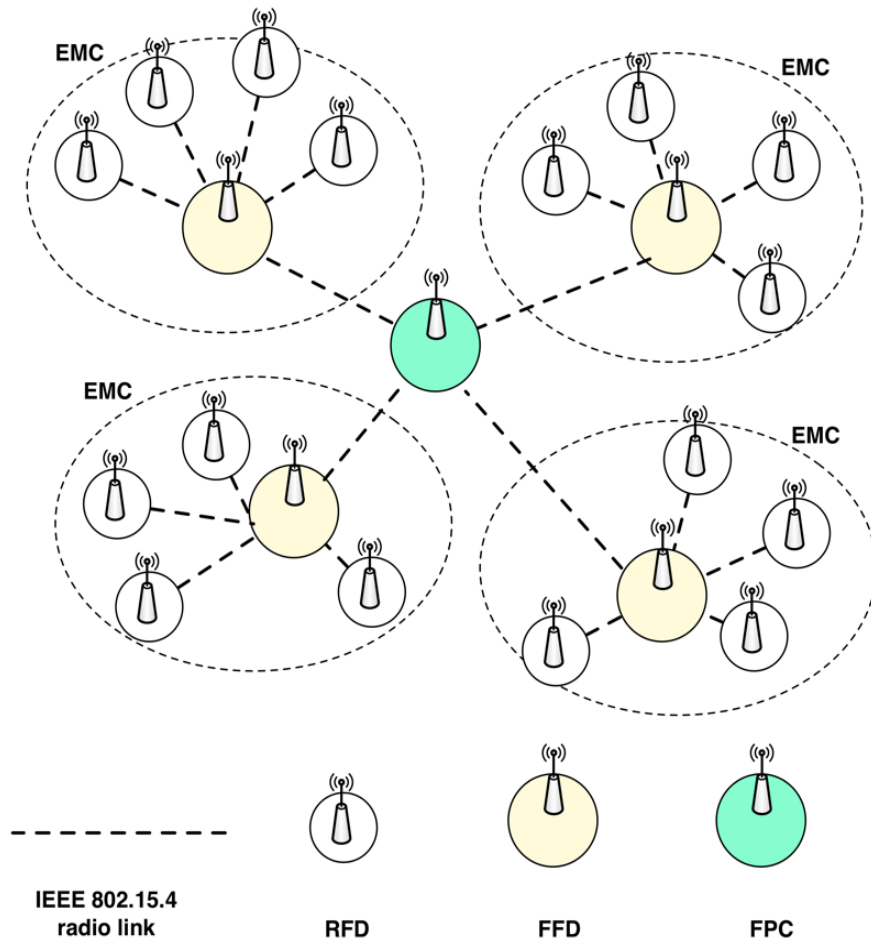
Fig. 1 Environmental monitoring IEEE 802.15.4 architecture
