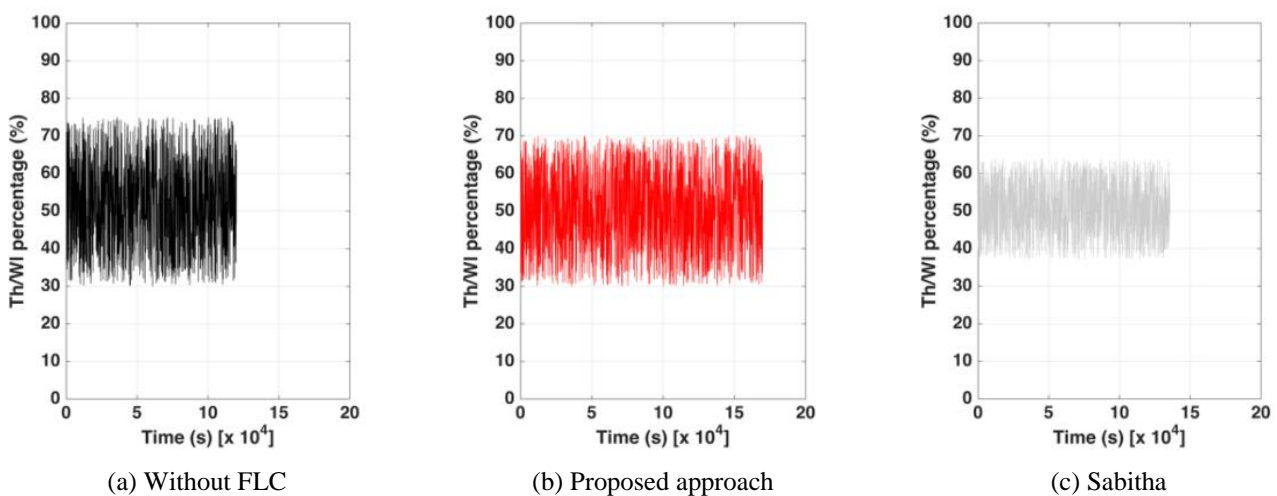
Fig. 8 Th/Wl behaviour on star topology [25]
