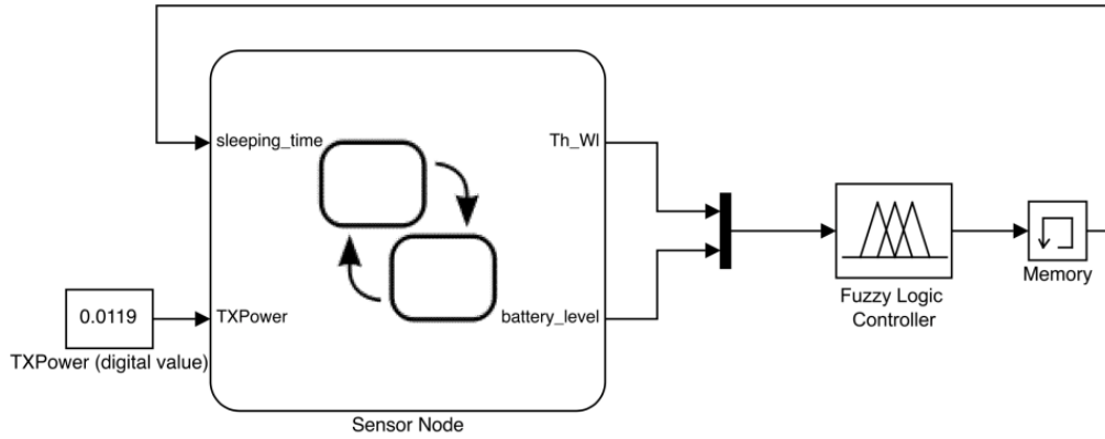
Fig. 5 Simulation model scheme
