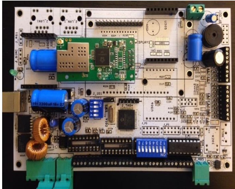
Fig. 4 Used prototyping board
