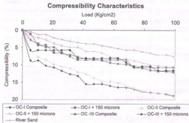
Fig.2 Compressibility of different overburden samples and river sand 100 kg/cm 2 (corresponding to a depth of 400m), of composite samples of OC-I, OC-II and OC-III OB samples are 18.9%, 19.09% and 12.02% respectively, which decreases to 10.72%, 10.58% and 11.52% respectively after washing the samples at 150 micron size. The corresponding value of compressibility for sand is 7.5%.
