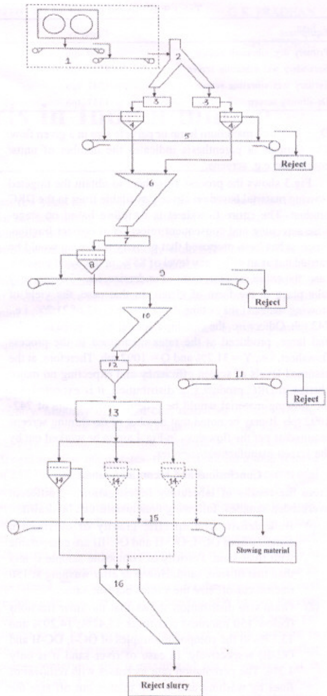
Fig.4 Material handling flow diagram based on already available fines in DRC product
