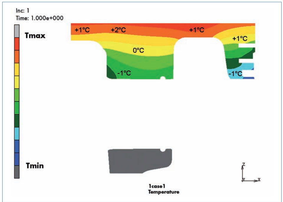
Fig. 23: Differences between temperature values obtained by FEM simulation and those estimated by the hardness tests in section X-X of Fig. 22.
