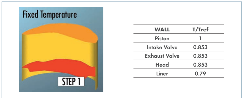
Fig. 3: Imposed wall temperature in the first step.
