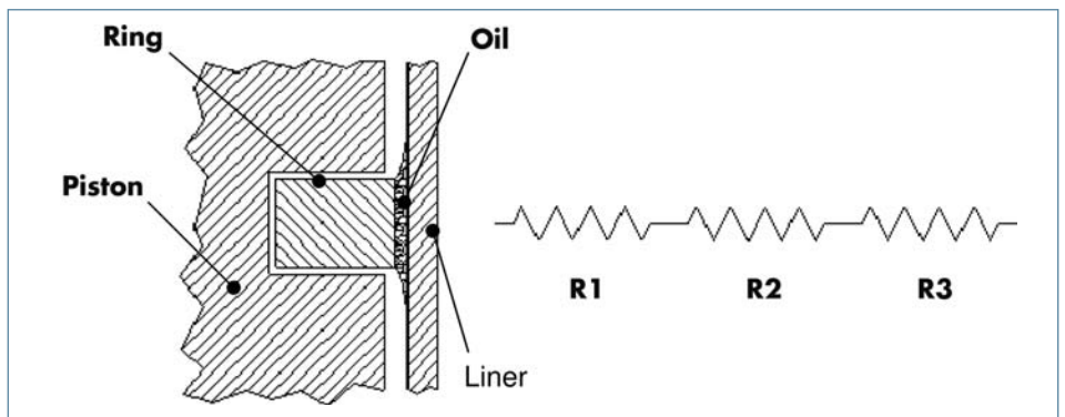
Fig. 8: Thermal resistance model of the rings.
