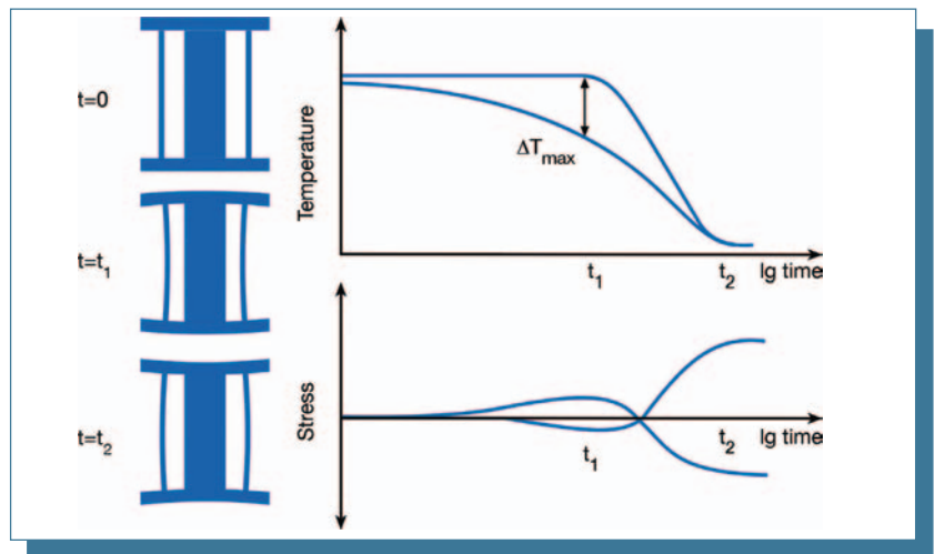
Fig. 1: Formation of residual stresses and distortion in a stress lattice
