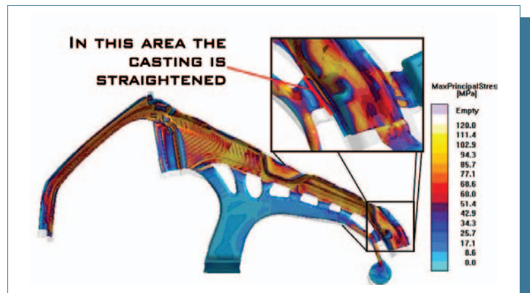
Fig. 3: Maximum Principle Stress in the rear door lock panel casting just before ejection. The original geometry is shown as semi transparent grey, as well as the deformed geometry showing the relative shape change and areas of contact and constraint.
