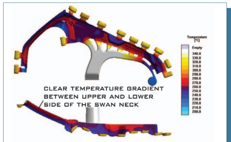
Fig. 4: Temperature distribution in the casting and runner at ejection.
