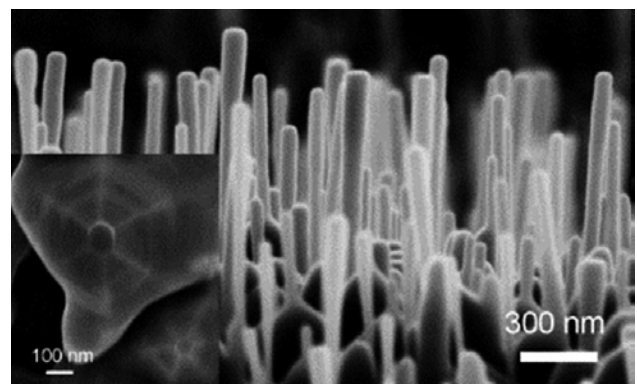
Fig. 1 - Cross-section FESEM image recorded at a 30° tilt angle showing diameter, length, and distribution of the as-grown ZnO NWs. Inset is a top-view showing the grown structure of the present ZnO NWs, which are hexagonal.
