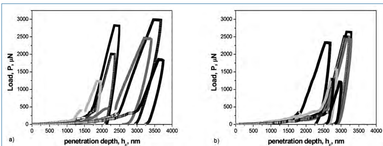
Fig. 3 - Six representative load-displacement nanoindentation curves showing the pop-in event upon loading of the ZnO NWs in the as-grown condition (maximum loads ranging 1.25- to - 3.0 mN), a), and after deep-cryogenic treatment (cooling to -196 °C at a rate of 1 °C/min, holding at -196 °C for 120 min, followed by 1 °C/min slow recover to room temperature), where maximum loads ranged 1.25-to-2.7 mN, b).
