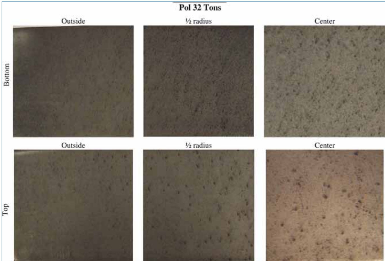
Fig. 9 - Macrostructure standard ingot (HCl 50% etch)
