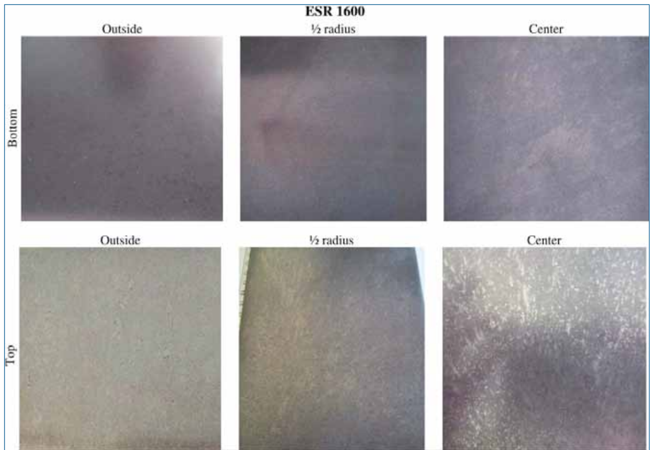
Fig. 8 - Macrostructure ESR ingot (HCl 50% etch)
