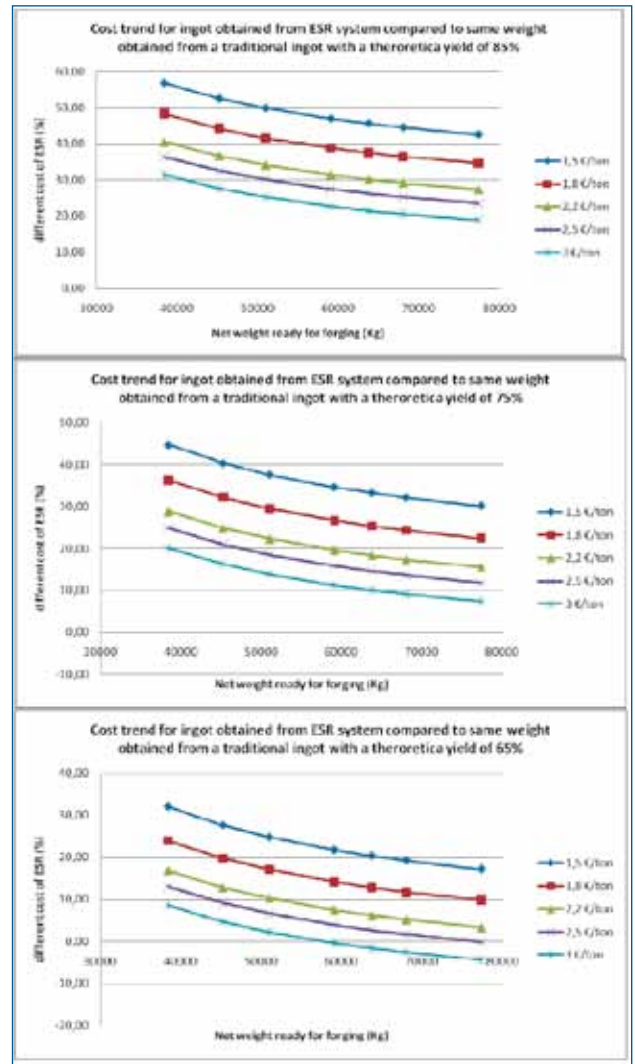
Fig. 10 - Graphs explaining economical behavior according to different parameters.
