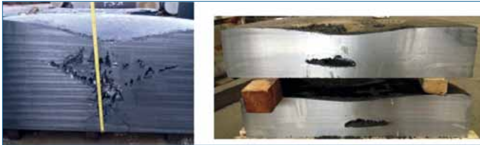
Fig. 3 - Examples of hot top cavities.
