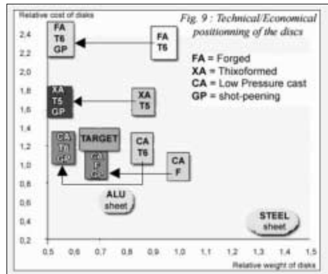
Fig. 9 - Technical/economical positioning of the disc.
