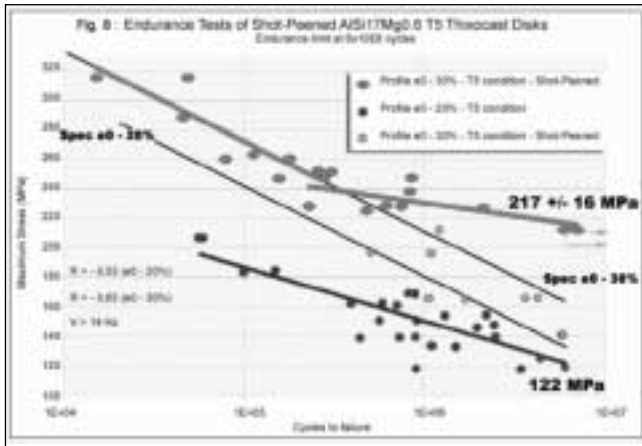
Fig. 8 - Endurance tests of shot peened AlSiMg 0.6 T5 thixocast discs.
