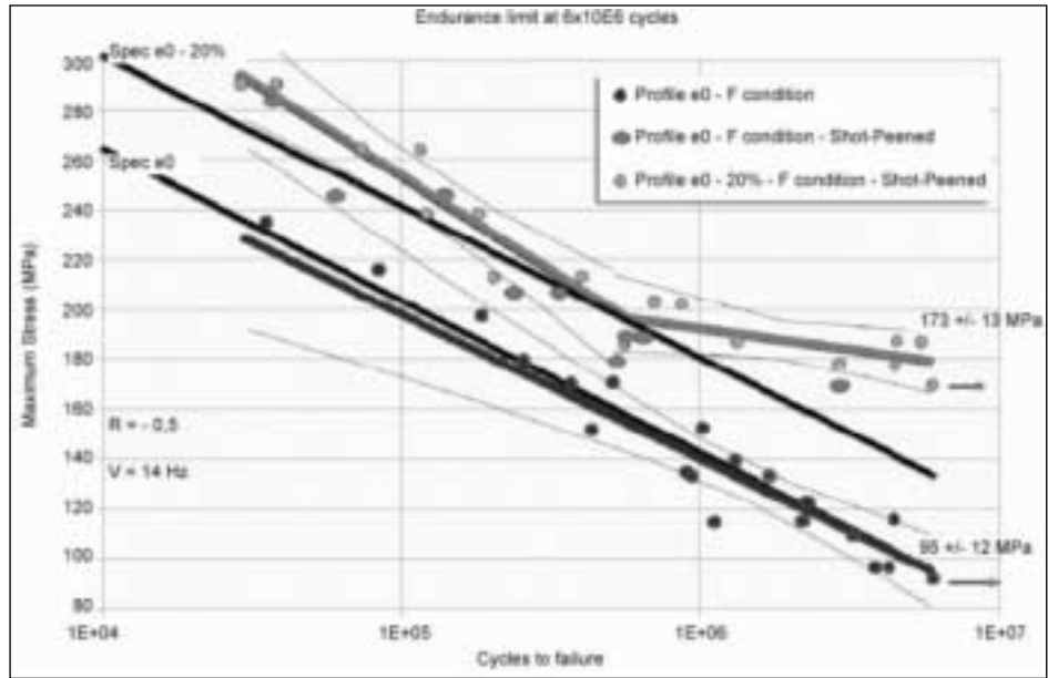
Fig. 11 – Endurance tests of shot-peened AlSi11Mg 0,2 F low pressure cast discs.
