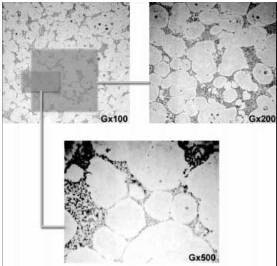
Fig. 6a – Thixoformed AlSi7Mg 0.6 T5 alloy disc. Globular structure of the primary phase \alpha -Al
