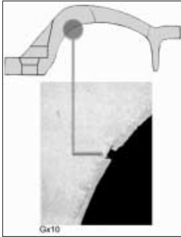
Fig. 5a – Thixoformed AlSi7Mg 0.6 T5 alloy disc. Poor adherence of the eutectic-rich skin.
