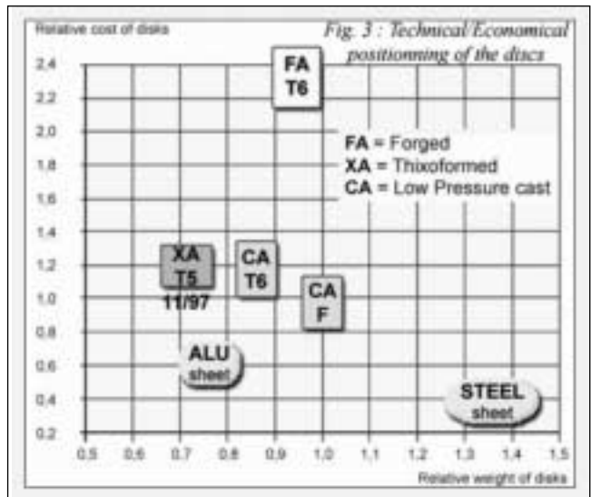
Fig. 3 – Technical/economical positioning of the disc.
