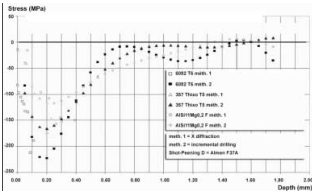
Fig. 10 – Residual stress measurements after shot peening.
