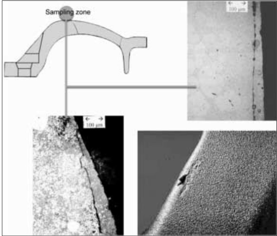
Fig. 5b – Thixoformed AlSi7Mg 0.6 T5 alloy disc. Poor adherence of the eutectic-rich skin.
