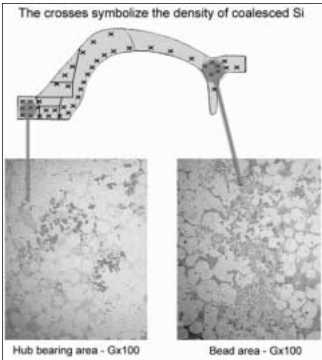
Fig. 7 – Thixoformed AlSi7Mg 0.6 T5 alloy disc. Coalesced silicon.
