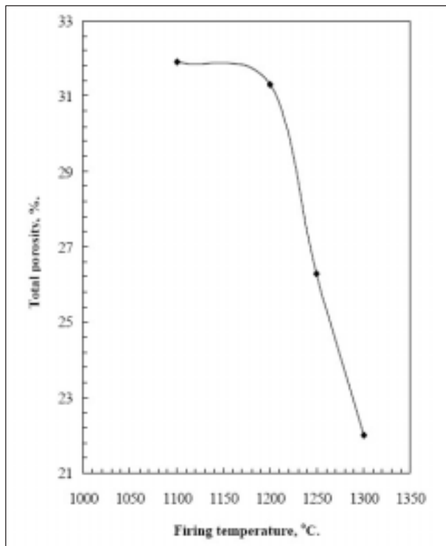
Fig. 6 – Effect of firing temperature on the total porosity of pellets containing 0.4% bentonite and 4% calcium hydroxide.
