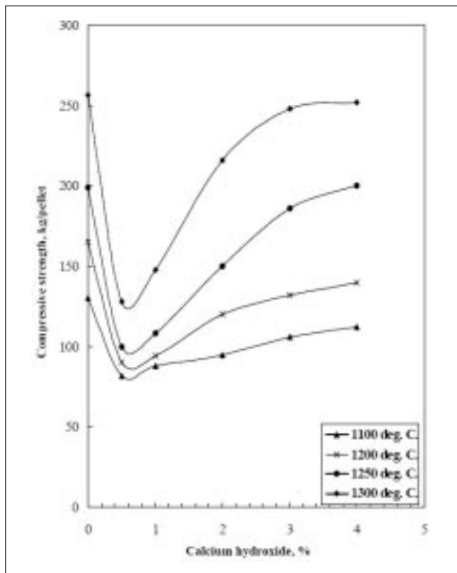
Fig. 3 – Effect of calcium hydroxide addition on the compressive strength of pellets fired at different firing temperatures and containing 0.4% bentonite.
