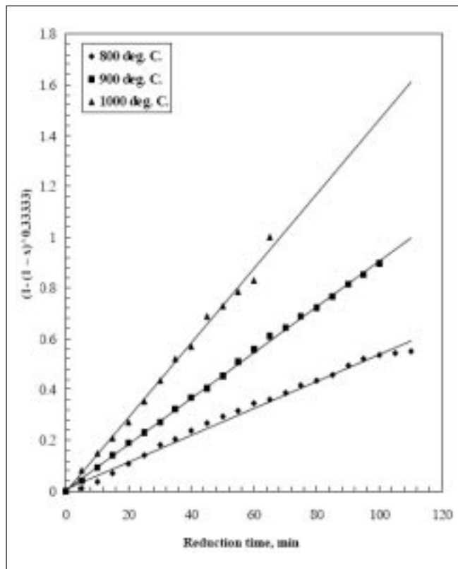
Fig. 9 – Relation between the time of reduction and (1 - (1-R)^{0.3333}) .
