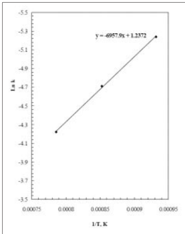
Fig. 10 – Arrhenius plot for the reduction of pellets containing 0.4 bentonite with 4% calcium hydroxide.
