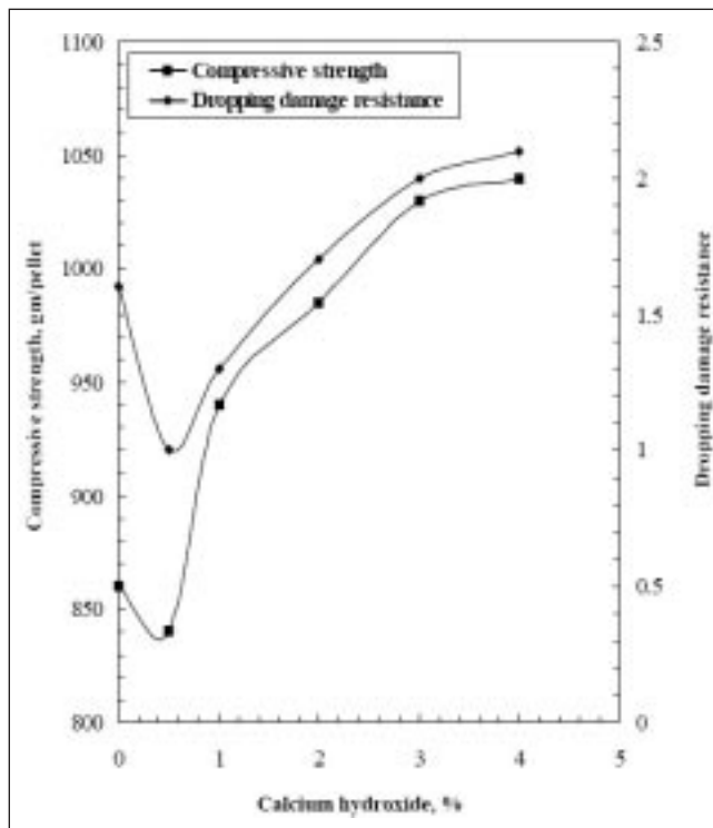
Fig. 1 – Effect of Calcium hydroxide addition on the mechanical properties of green pellets containing 0.4% bentonite.
