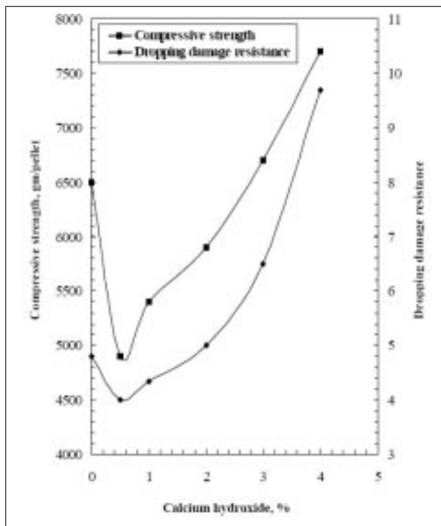
Fig. 2 – Effect of calcium hydroxide addition on the mechanical properties of dried pellets containing 0.4% bentonite.
