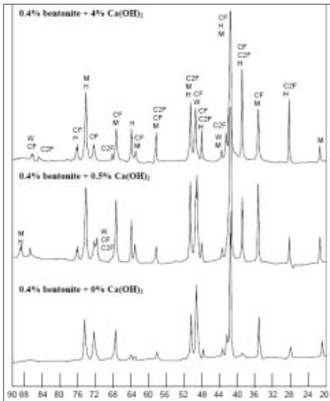
Fig. 5 – XRD of pellets containing different contents of calcium hydroxide with 0.4% bentonite and fired at 1300 °C.
