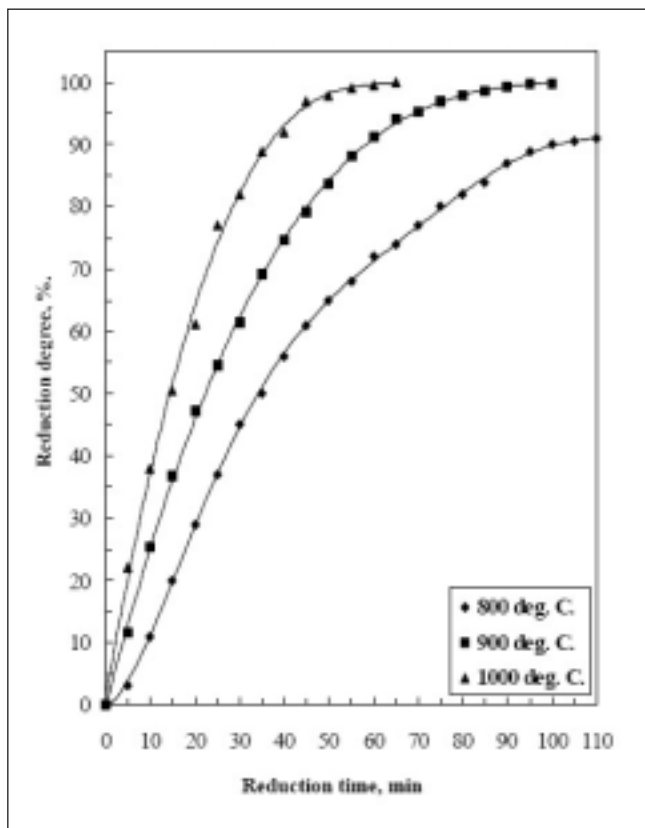
Fig. 8 – Effect of reduction temperature on the reduction degree of pellets containing 0.4% bentonite with 4% calcium hydroxide.
