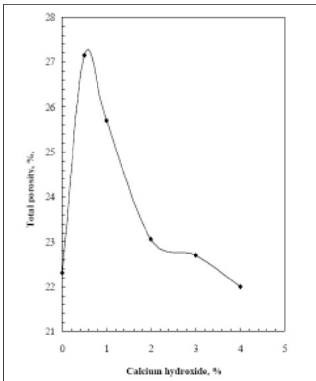
Fig. 4 – Effect of calcium hydroxide addition on the total porosity of pellets fired at 1300 °C and containing 0.4% bentonite.
