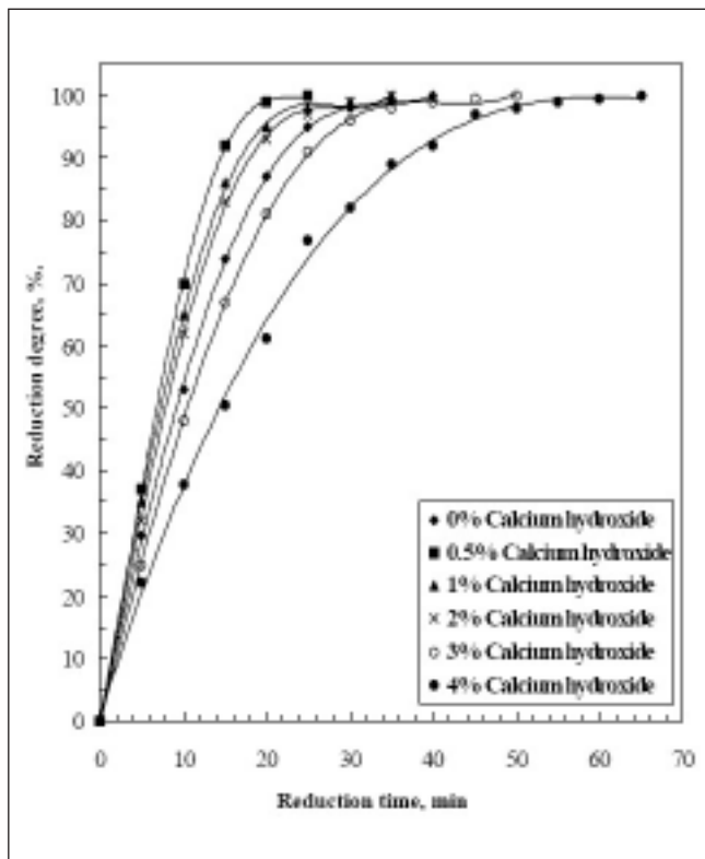
Fig. 7 – Effect of calcium hydroxide addition on the reducibility of pellets fired at 1300 °C and containing 0.4% bentonite.
