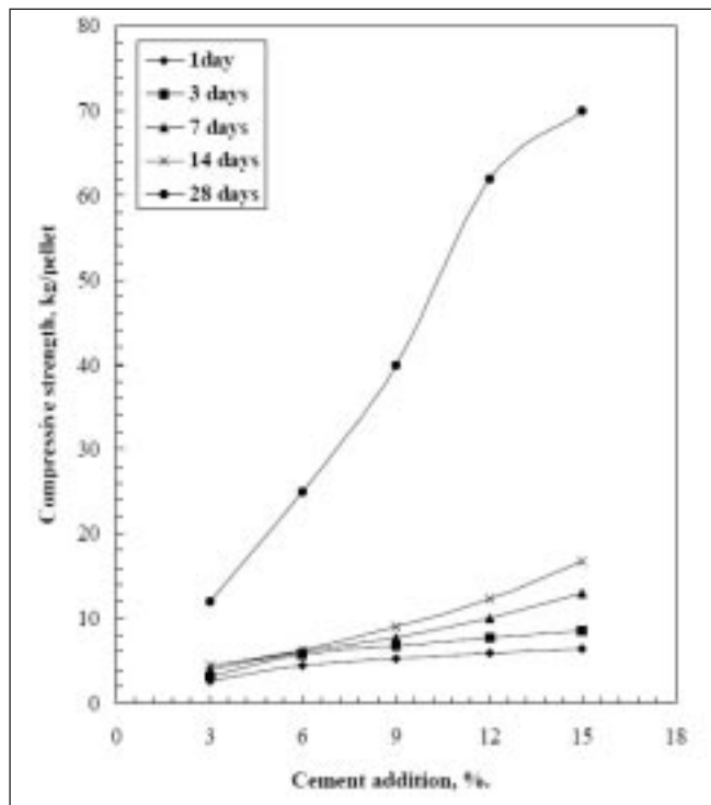
Fig. 5 – Effect of cement addition on the compressive strength of pellets cured at different curing periods, (water amount = 10%).
