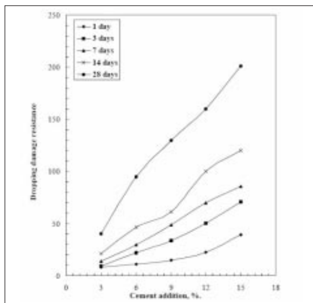
Fig. 4 – Effect of cement addition on the dropping damage resistance of pellets cured at different curing periods, (water amount = 13%).
