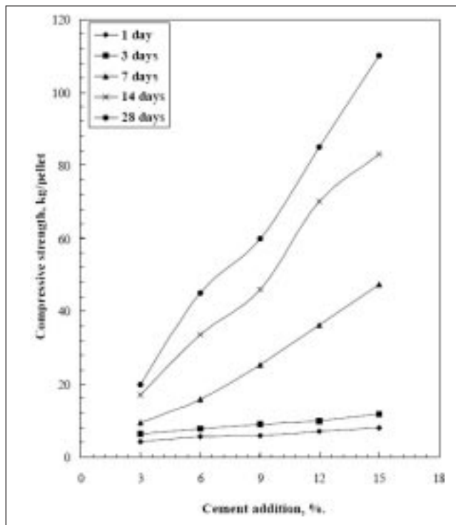
Fig. 6 – Effect of cement addition on the compressive strength of pellets cured at different curing periods, (water amount = 13%).
