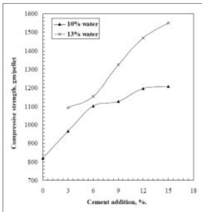
Fig. 2 – Effect of cement addition on the compressive strength of green pellets.
