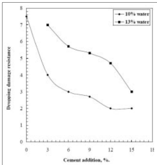
Fig. 1 – Effect of cement addition on the dropping damage resistance of green pellets.
