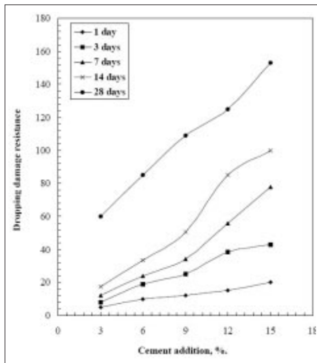
Fig. 3 – Effect of cement addition on the dropping damage resistance of pellets cured at different curing periods, (water amount = 10%).
