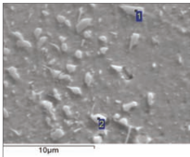
FIG. 3 WDS image of high N cast, coarse grained and aged for 2000 h at 800 °C.
