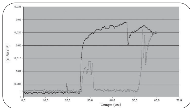
Fig. 11 Test cronopotentiostatico in 0.2 M NaCl. Chronopotentiostatic test in 0.2 M NaCl.
