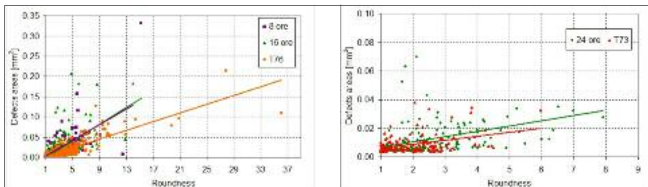
FIG. 6 Roundness versus defects areas.
