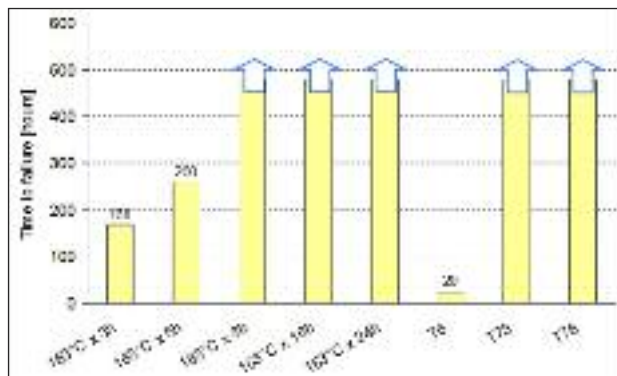
FIG. 4 SCC resistance in the salt fog chamber (480 hours maximum exposure time).
