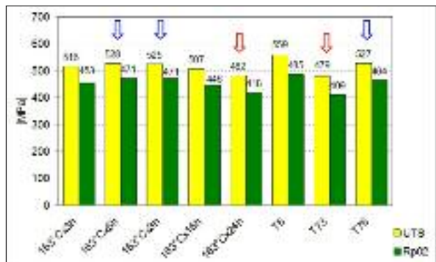
Fig. 3 Tensile results for the investigated heat treatment conditions.
