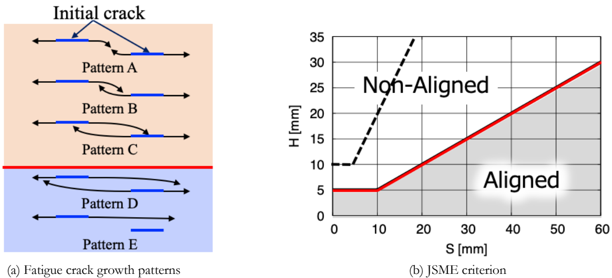
Figure 3: (a) Fatigue crack growth patterns of two non-coplanar cracks and (b) the alignment rule given by the Japan Society for Mechanical Engineers (JSME). The red bold line in the right figure is determined by the experiments of the fatigue crack growth of surface cracks. Finite element mesh for the fatigue crack growth simulation of two non-coplanar embedded cracks. Each crack. The alignment rule is defined by the horizontal separation S and the vertical height H . The JSME criterion fully covers the area defined by the bold red line.
