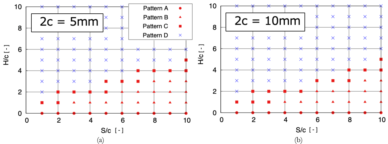
Figure 7: Interaction map of two non-coplanar embedded cracks obtained by the s-FEM simulations. The initial crack sizes are (a) 2c=5 mm and (b) 2c=10 mm. The plot is based on the length of H and S normalized by the half size of crack c . The borders determined by the JSME and Ando et al. are also plotted.
