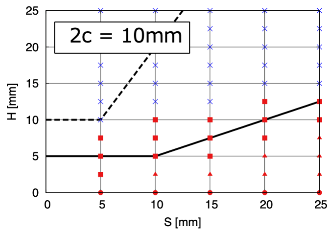
Figure 6: Interaction map of two non-coplanar embedded cracks obtained by the s-FEM simulations. The initial crack size is 2c=10 mm. The plot is based on the real length of H and S . The borders determined by the JSME and Ando et al. are also plotted.
