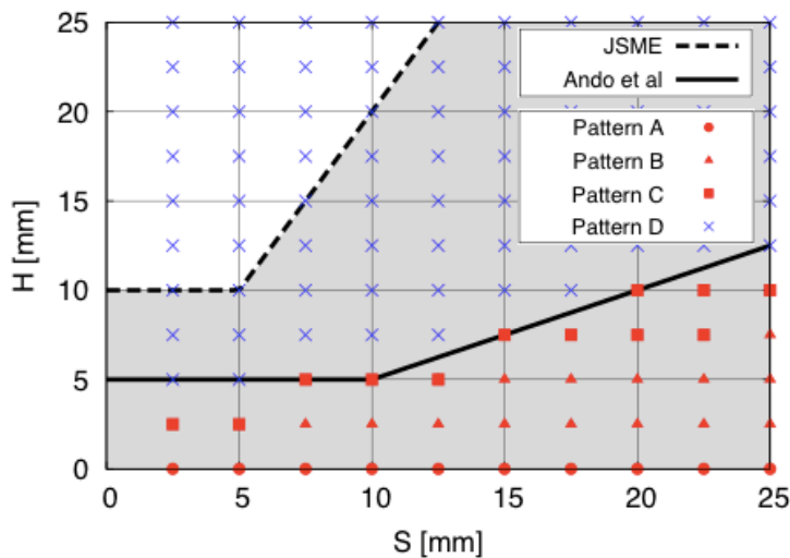
Figure 5: Interaction map of two non-coplanar embedded cracks obtained by the s-FEM simulations. The marks shows the fatigue crack growth patterns. The borders determined by the JSME and Ando et al. are also plotted.
