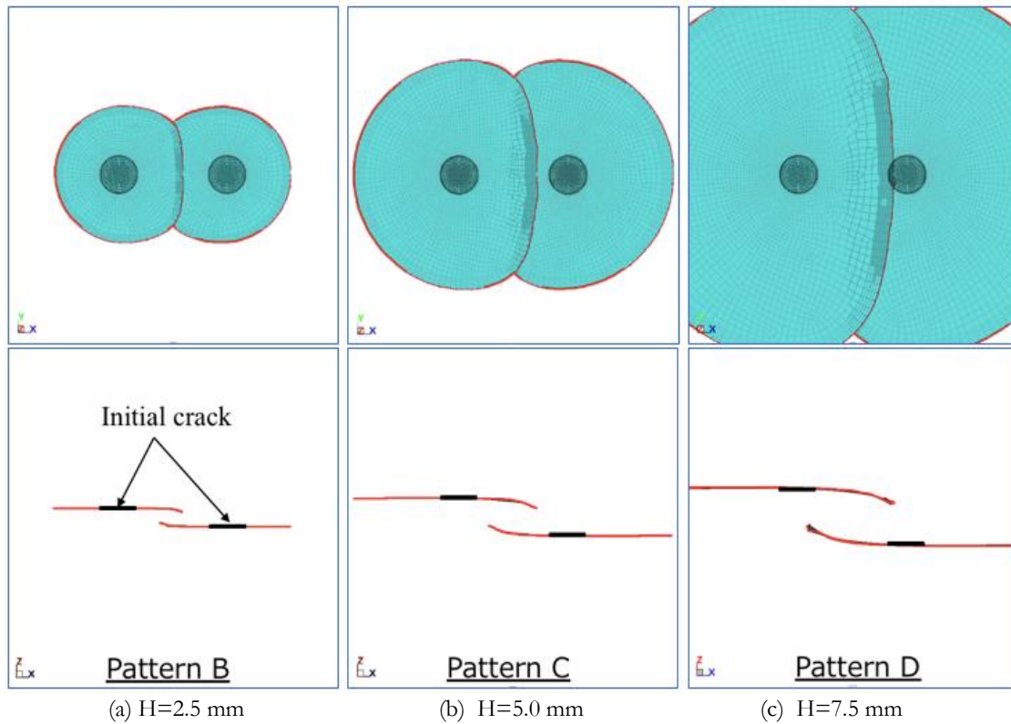
Figure 4: Fatigue crack growth behavior of two non-coplanar embedded cracks. The horizontal separation S of the initial crack tips is 10 mm, and the vertical height H is (a) 2.5 mm, (b) 5.0 mm and (c) 7.5 mm. Only crack shape is displayed. The red line shows the crack tip. The top figure is the top view of the crack shape, and the bottom figure is the front view of the crack shape. The crack growth behavior is categorized into (a) pattern B, (b) pattern C, and (c) pattern D, respectively.
