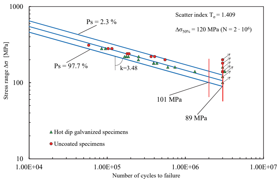
Figure 8: Unified scatterband considering uncoated and hot dip galvanized connections.
