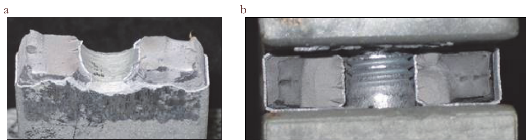
Figure 5: Typical fracture surface after cyclic loading. (a) Plate and (b) bolted part.
