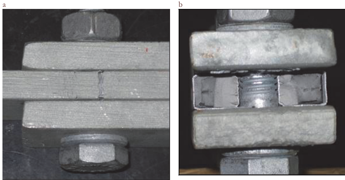
Figure 4: Typical failure from the hole corresponding to the first bolt of the connection. (a) lateral view and (b) upper view.
