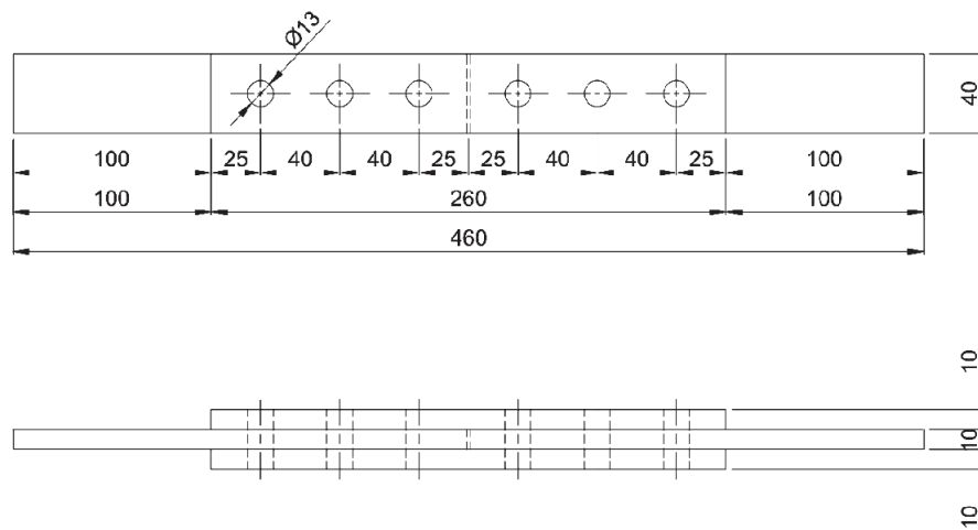
Figure 1: Geometry of the test specimen employed in the research program.
