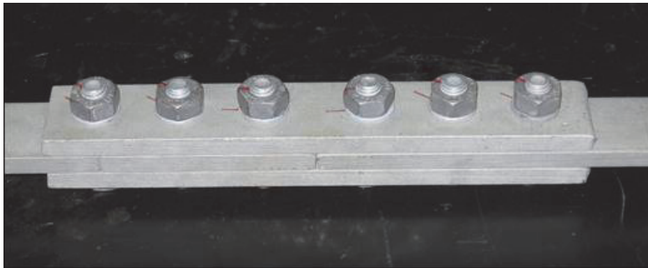
Figure 2: Hot-dip galvanized bolted connection before the test.
