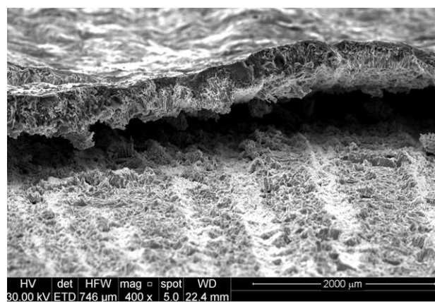
Figure 6: Layer thickness from a SEM image.
