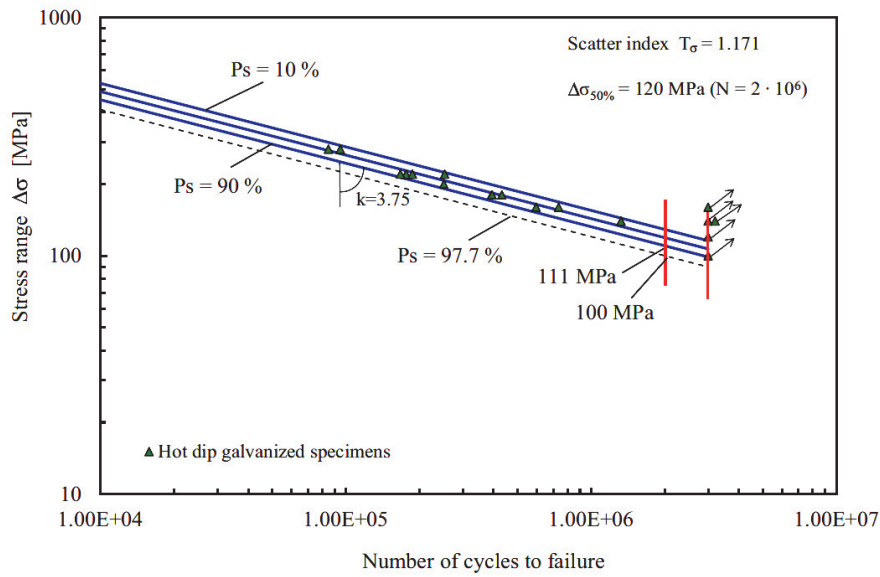
Figure 7: S-N-curves of hot dip galvanized connections.
