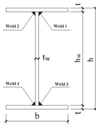
Figure 2: Specimens sizes
