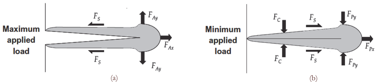
Figure 3: Forces between the plastic enclave (grey), and the surrounding elastic material (after [7]).
