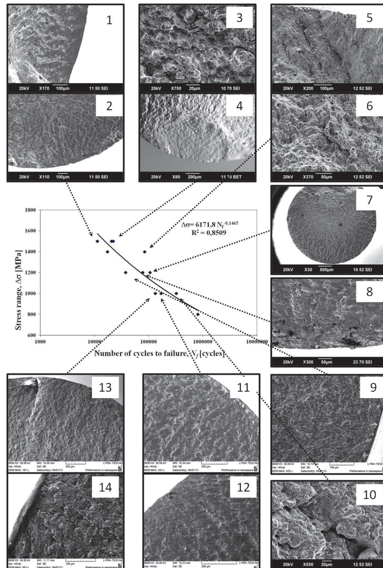
Figure 3: Wöhler curve of Steel A and characteristic areas of the fractured specimen surfaces corresponding to some stress ranges.
