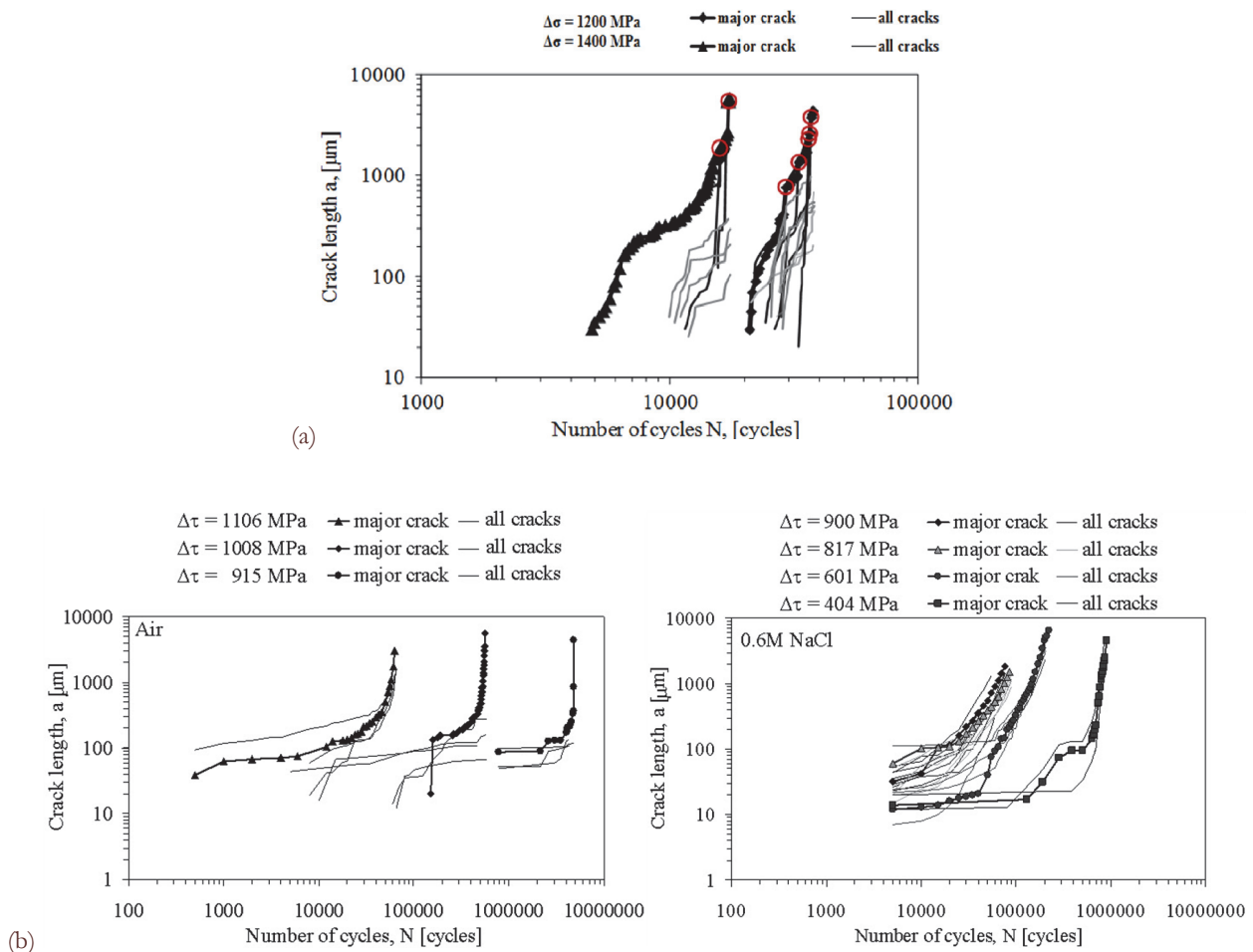
Figure 6: Presentation "Crack length, a - Numbers of cycles, N ": (a) Steel A, Specimen 7 ( \Delta\sigma = 1200 MPa) and Specimen 9 ( \Delta\sigma = 1400 MPa); (b) Steel B, Specimen sets tested in-air and corrosion environment.
