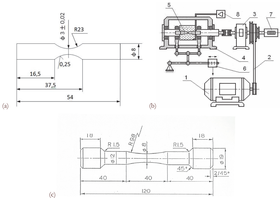
Figure 2: Specimen geometry and fatigue equipment: (a) steel A specimen; (b) fatigue machine FATROBEM 2004; (c) Steel B specimen; FATROBEM 2004 - electric engine 1, driving belt 2, ball-bearing unit 3, testing box 4, specimen 5, device for loading 6, counter 7, device for circulation and aeration of corrosion agent 8.
