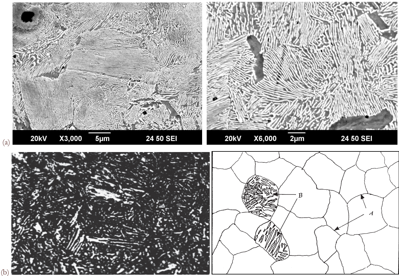
Figure 1: Microstructures of: (a) Steel A; (b) Steel B with schematic presentation (A-Prior austenite grain boundaries, B-Martensite laths).
