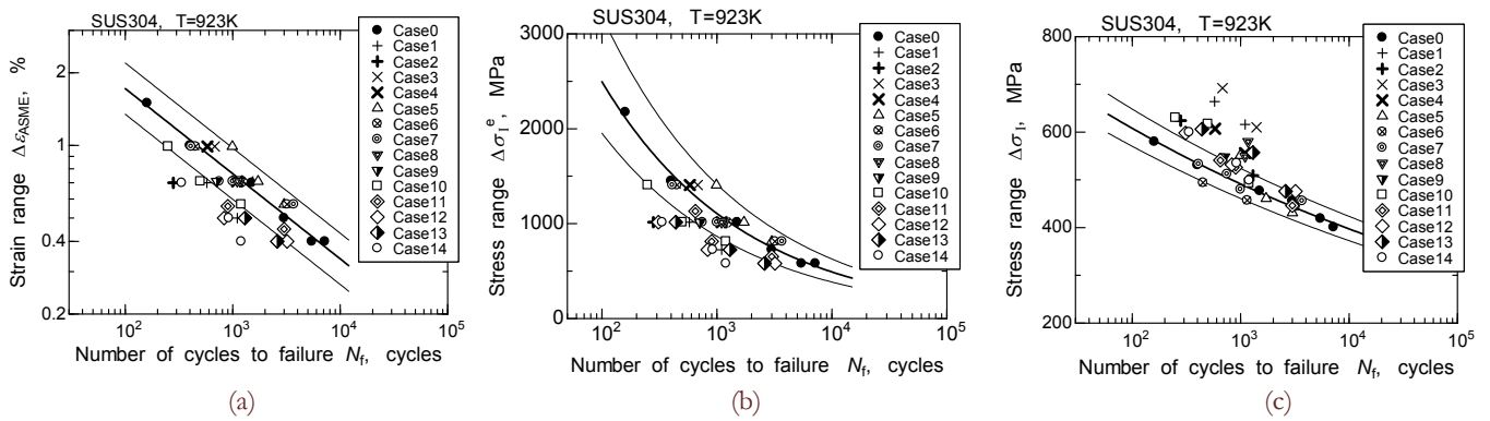
Figure 9: Correlation of non-proportional LCF lives with \Delta\epsilon_{ASME} , \Delta\sigma_I^e and \Delta\sigma_I : (a) \Delta\epsilon_{ASME} - N_f , (b) \Delta\sigma_I^e - N_f , (c) \Delta\sigma_I - N_f .
