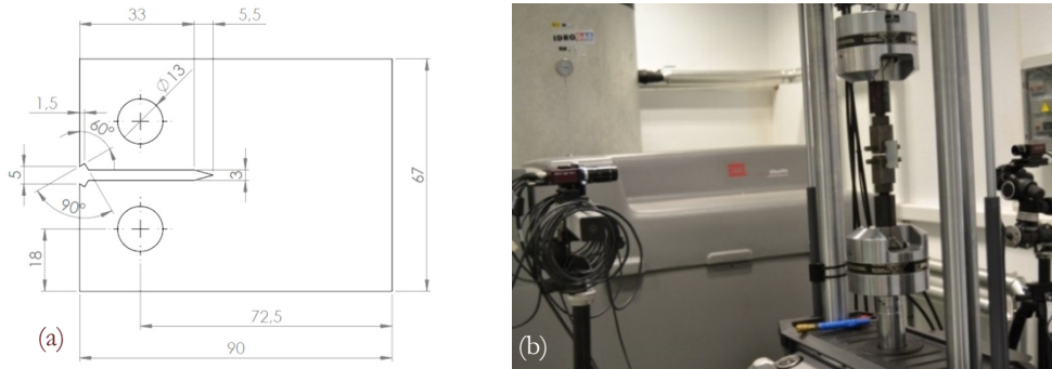
Figure 2: CT specimen (a) and experimental set-up (b) used for fatigue testing.
