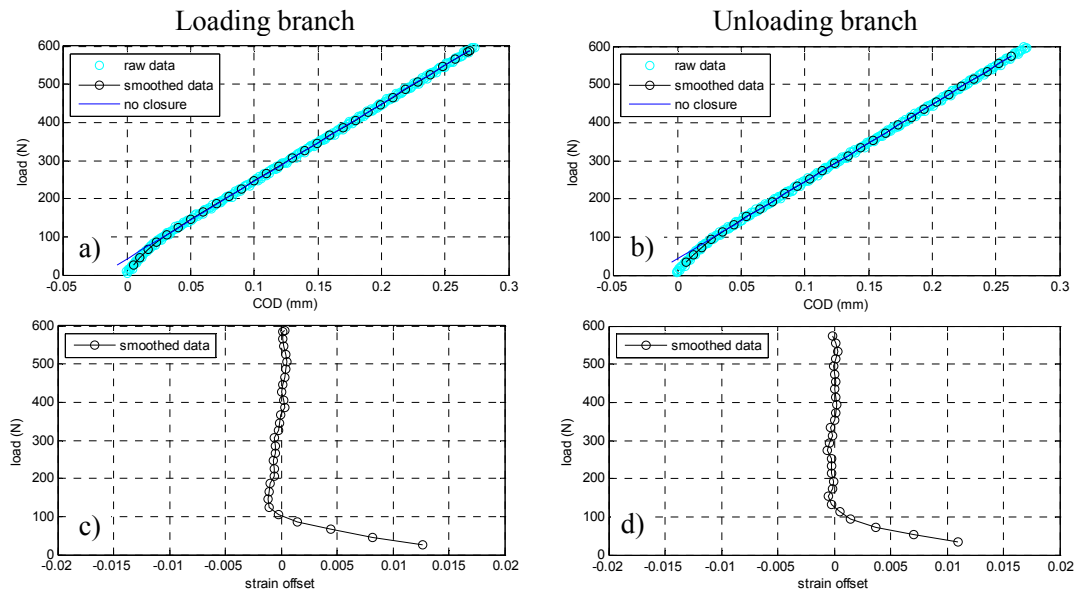
Figure 7: Results obtained from strain offset method for a crack length of 35.47 mm corresponding to the specimen tested at low R -ratio. a) Applied load versus COD for loading branch, b) applied load versus COD for unloading branch, c) applied load versus strain offset for loading branch and d) applied load versus strain offset for unloading branch.
