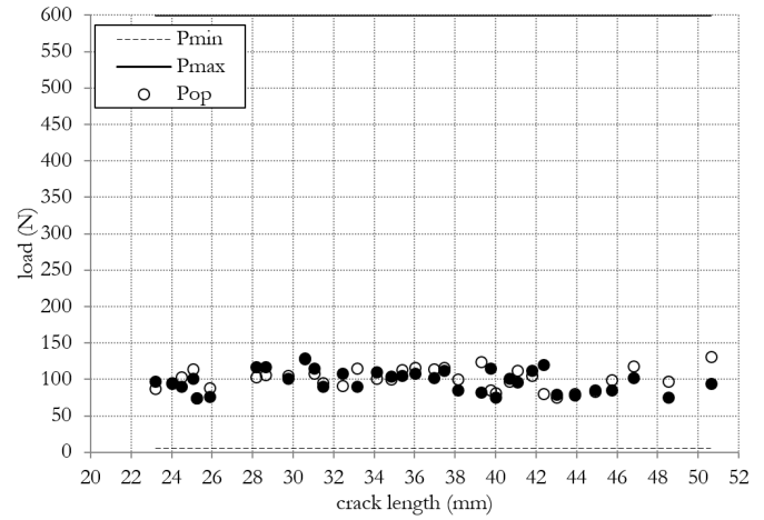
Figure 6: P_{op} and P_{cl} at different crack lengths for the specimen tested at low R -ratio.
