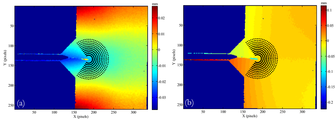
Figure 3: Horizontal (a) and vertical (b) displacement fields measured for a 34.10 mm and a load level of 600 N.
