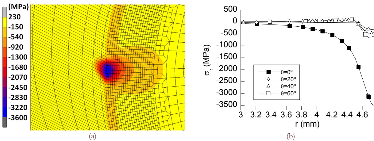
Figure 2: Distribution of radial stress after the sixth loading cycle: (a) 3D view at the contact of one of the balls and (b) radial distribution for diverse hoop coordinates \theta .
