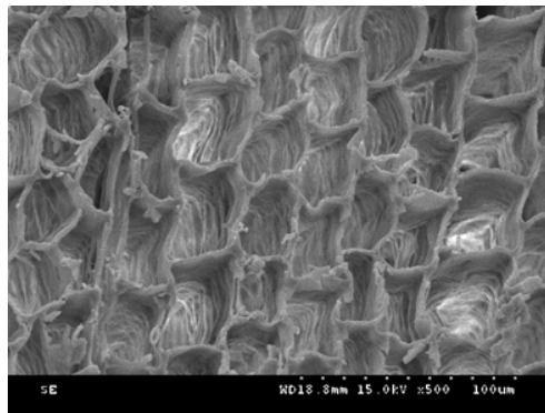
(a) 500×waterlogged wood SEM microstructure of early wood cells on cross section
