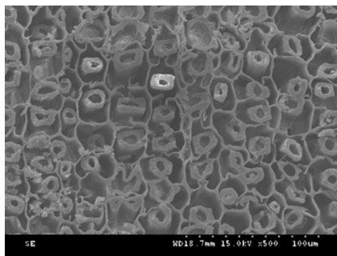
(b) 500×waterlogged wood SEM microstructure of late wood on cross section
