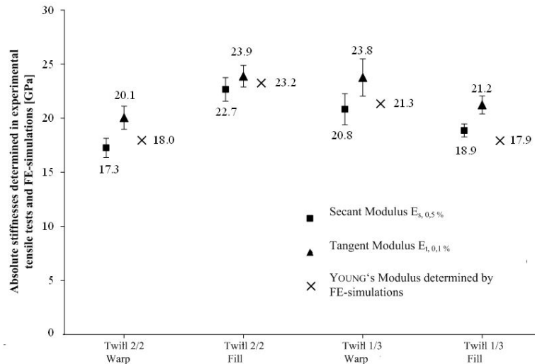
Figure 9: Secant modulus and tangent modulus of the respective textile semi-finished products based on the experimentally determined values of the fibre volume content of \varphi_f .
