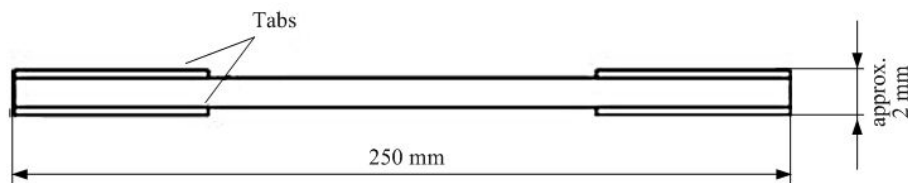
Figure 3: Side view of the tensile test specimens with tabs according to German standard DIN EN 2747 [7].
