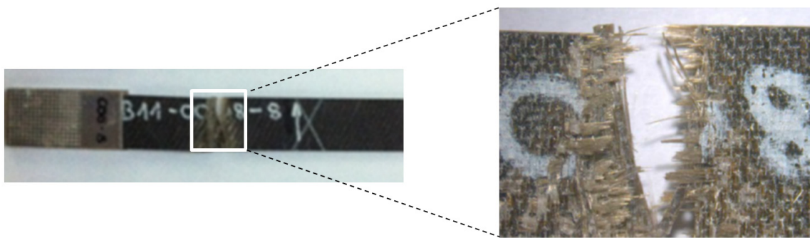
Figure 11: Fractured specimen with twill weave 2/2 fabric reinforcement in the warp direction. The area enclosed in the square box show details of the damage mechanism.
