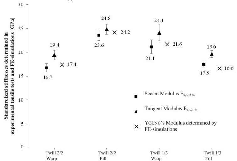
Figure 10: Secant modulus and tangent modulus of the respective textile semi-finished products standardized to a fibre volume content of \varphi_f=50\% .
