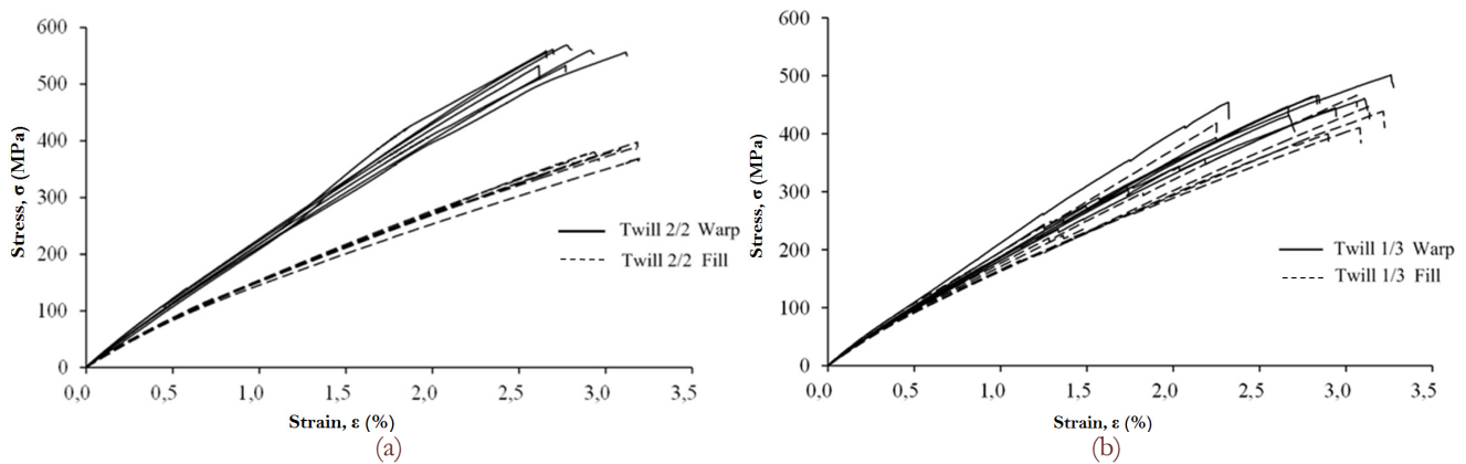
Figure 8: Stress-strain diagrams as results of the experimental tensile tests: (a) fabric type twill 2/2 in warp and fill direction; (b) Fabric type twill 1/3 in warp and fill direction.
