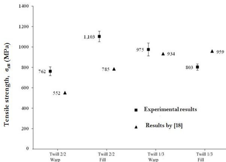
Figure 12: Calculated tensile strengths of the respective textile semi-finished products standardized to a fibre volume content of \varphi_f=50\% .
