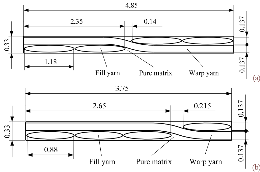
Figure 4: Schematic depiction of sample cross-sections for the two types of dry fabric reinforcements. (a) Twill wave 2/2; (b) Twill weave 1/3.
