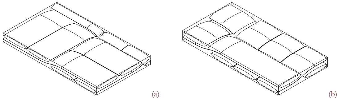
Figure 5: 3D models of the RVE. (a) Twill weave 2/2; (b) Twill weave 1/3.
