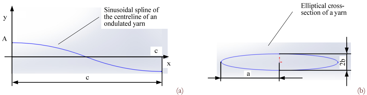
Figure 6: Simplifying assumptions for analytical description of the geometry: (a) Sinusoidal spline about centreline of an undulated yarn; (b) Elliptical cross-section of a yarn.
