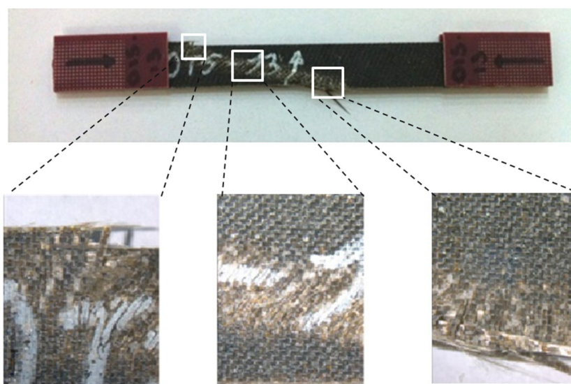
Figure 13: Fractured specimen with twill weave 1/3 fabric reinforcement in the fill direction. The areas enclosed in the square boxes show details of the damage mechanism leading to sample failure.
